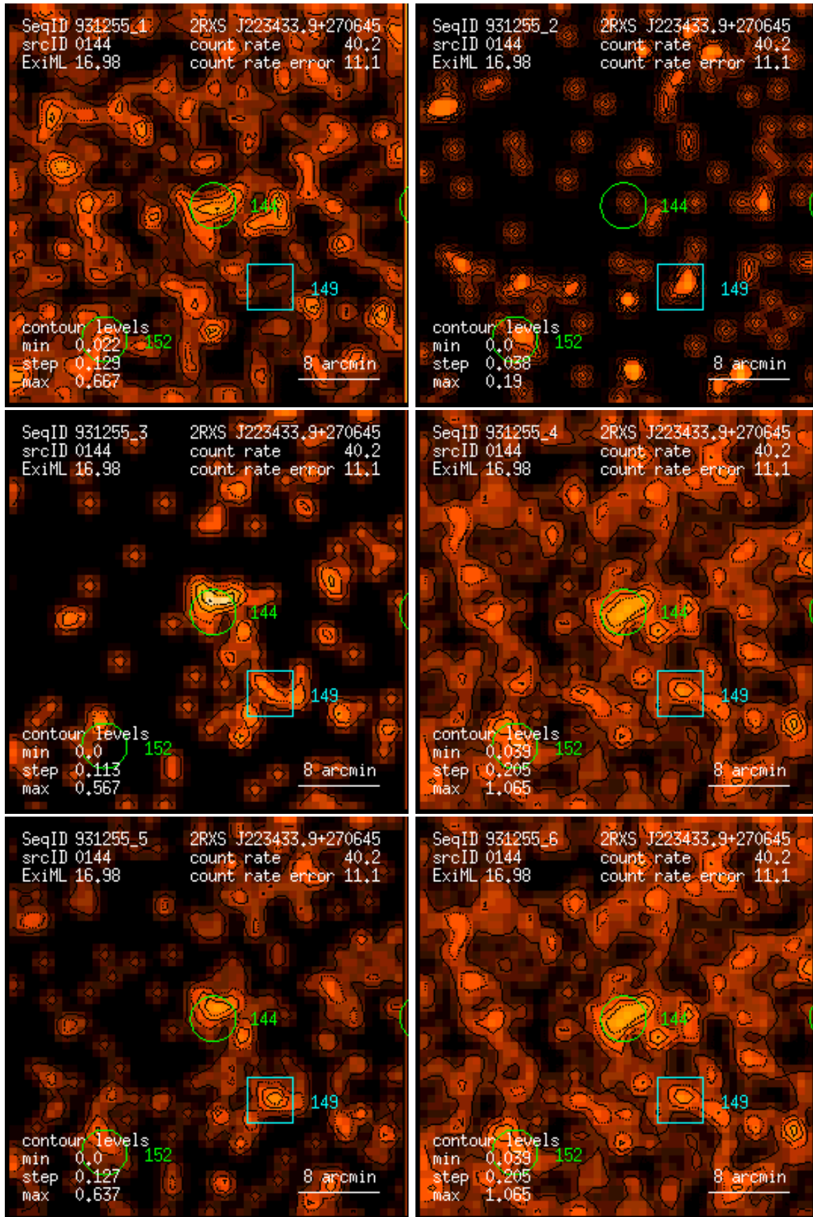
Figure 144: RASS 931255: detection 0144: band rate images, Gaussian filter: (1) PSPC channels 11 – 41, (2) 52 – 90, (3) 91 – 201, (4) 11 – 235, (5) 52 – 201, (6) 11 – 201. Broad band rates in counts/ks. Band rate contour levels in counts/ks/arcmin 2 .
