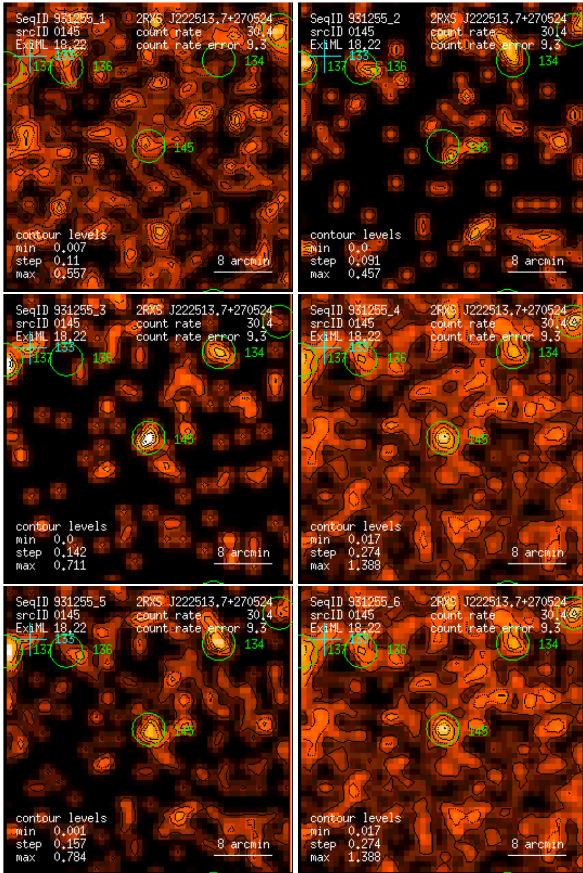
Figure 145: RASS 931255: detection 0145: band rate images, Gaussian filter: (1) PSPC channels 11 – 41, (2) 52 – 90, (3) 91 – 201, (4) 11 – 235, (5) 52 – 201, (6) 11 – 201. Broad band rates in counts/ks. Band rate contour levels in counts/ks/arcmin 2 .
