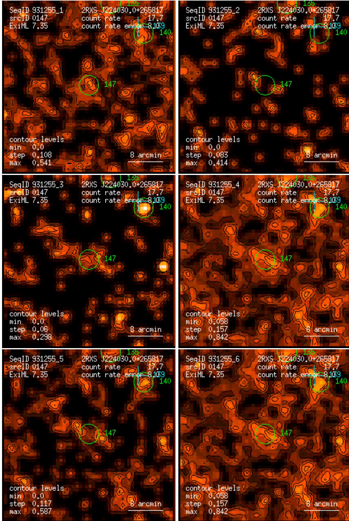
Figure 147: RASS 931255: detection 0147: band rate images, Gaussian filter: (1) PSPC channels 11 – 41, (2) 52 – 90, (3) 91 – 201, (4) 11 – 235, (5) 52 – 201, (6) 11 – 201. Broad band rates in counts/ks. Band rate contour levels in counts/ks/arcmin 2 .
