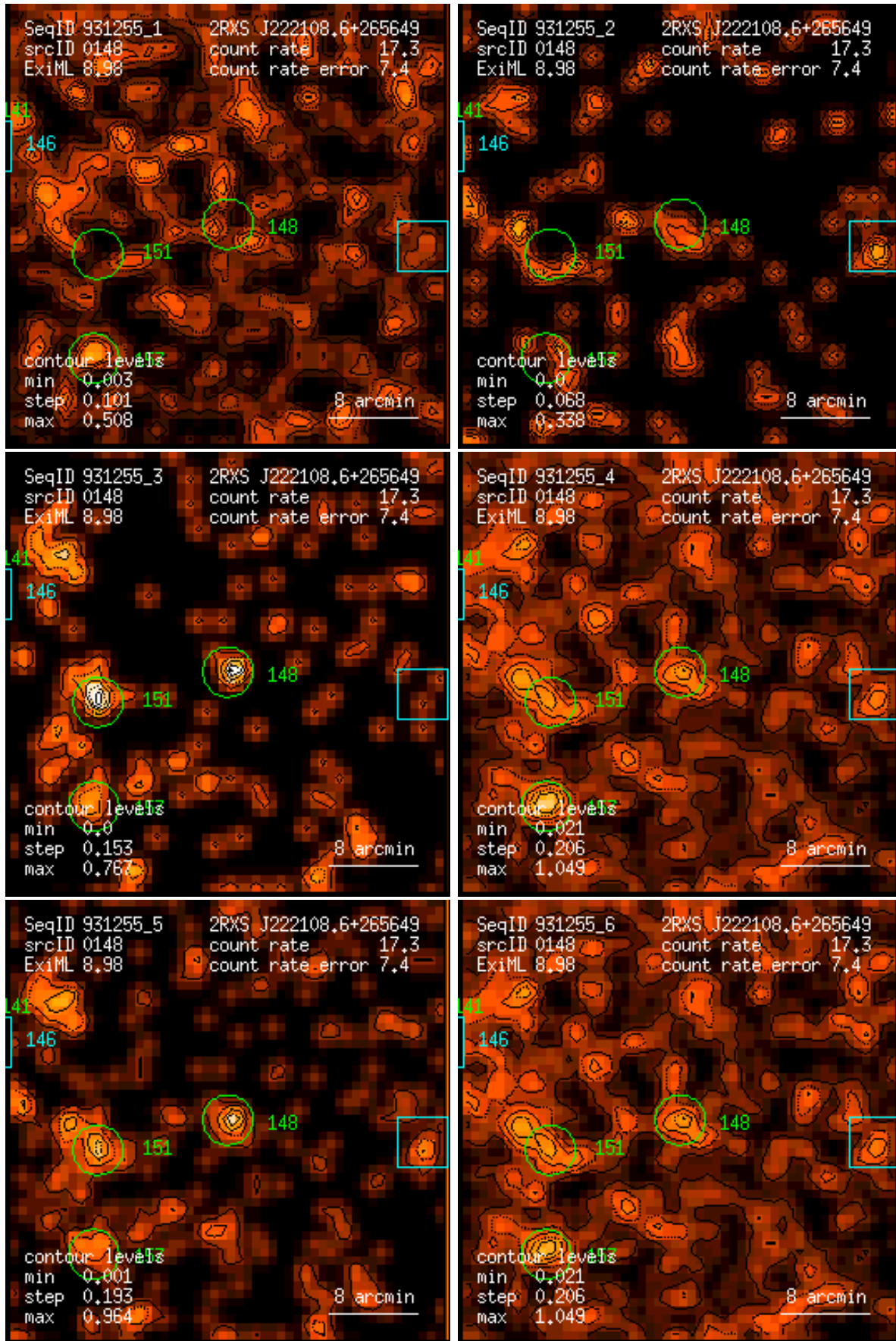
Figure 148: RASS 931255: detection 0148: band rate images, Gaussian filter: (1) PSPC channels 11 – 41, (2) 52 – 90, (3) 91 – 201, (4) 11 – 235, (5) 52 – 201, (6) 11 – 201. Broad band rates in counts/ks. Band rate contour levels in counts/ks/arcmin 2 .
