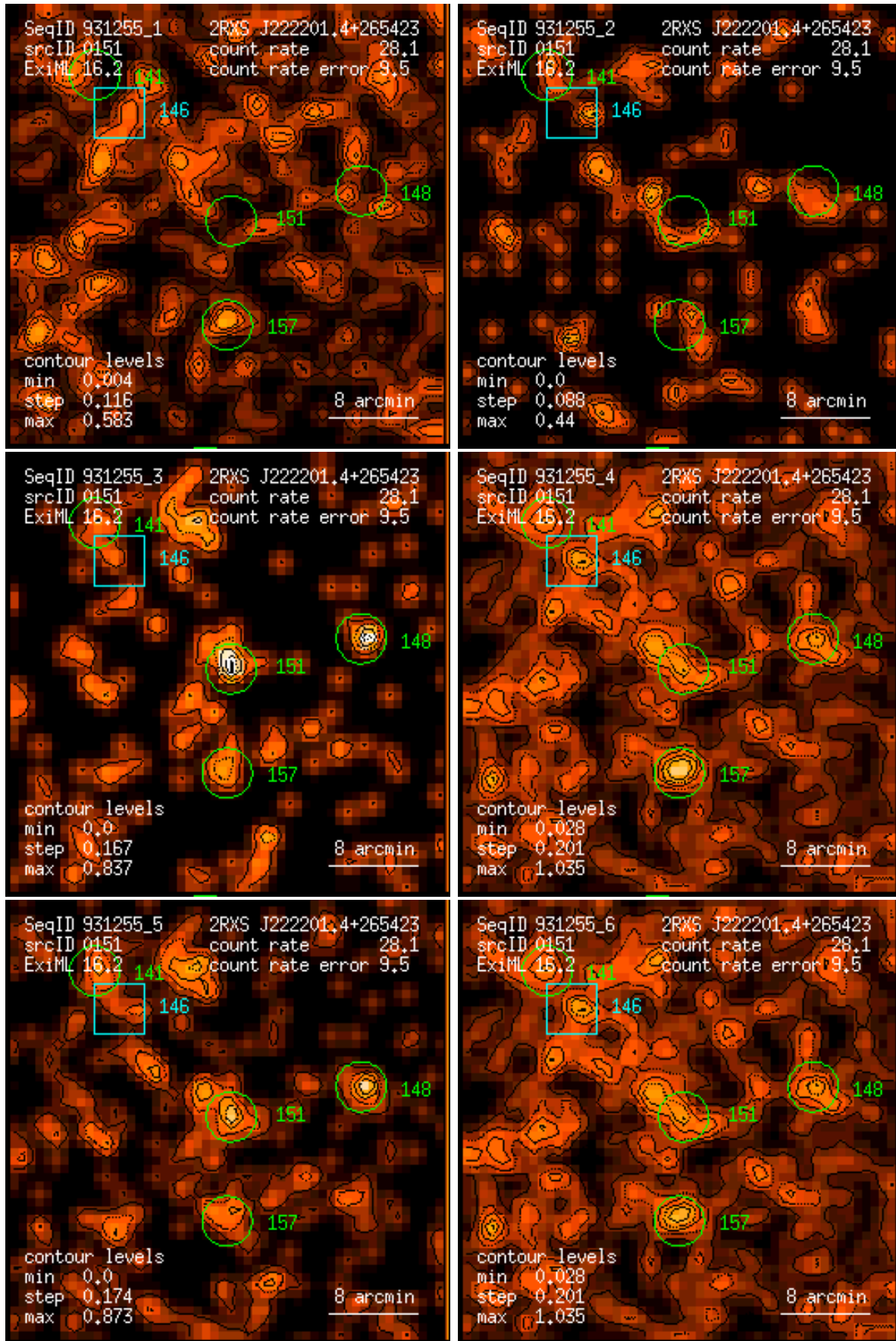
Figure 151: RASS 931255: detection 0151: band rate images, Gaussian filter: (1) PSPC channels 11 – 41, (2) 52 – 90, (3) 91 – 201, (4) 11 – 235, (5) 52 – 201, (6) 11 – 201. Broad band rates in counts/ks. Band rate contour levels in counts/ks/arcmin 2 .
