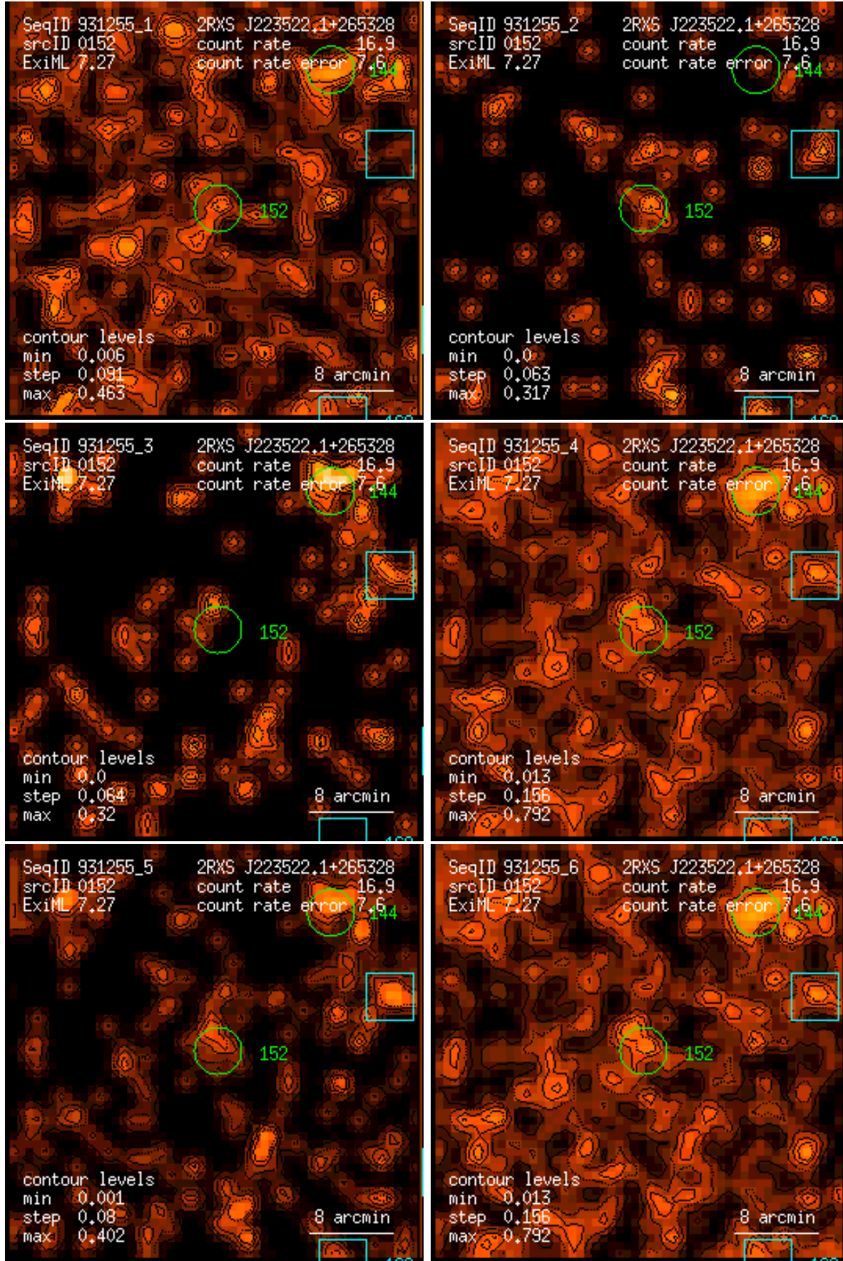
Figure 152: RASS 931255: detection 0152: band rate images, Gaussian filter: (1) PSPC channels 11 – 41, (2) 52 – 90, (3) 91 – 201, (4) 11 – 235, (5) 52 – 201, (6) 11 – 201. Broad band rates in counts/ks. Band rate contour levels in counts/ks/arcmin 2 .
