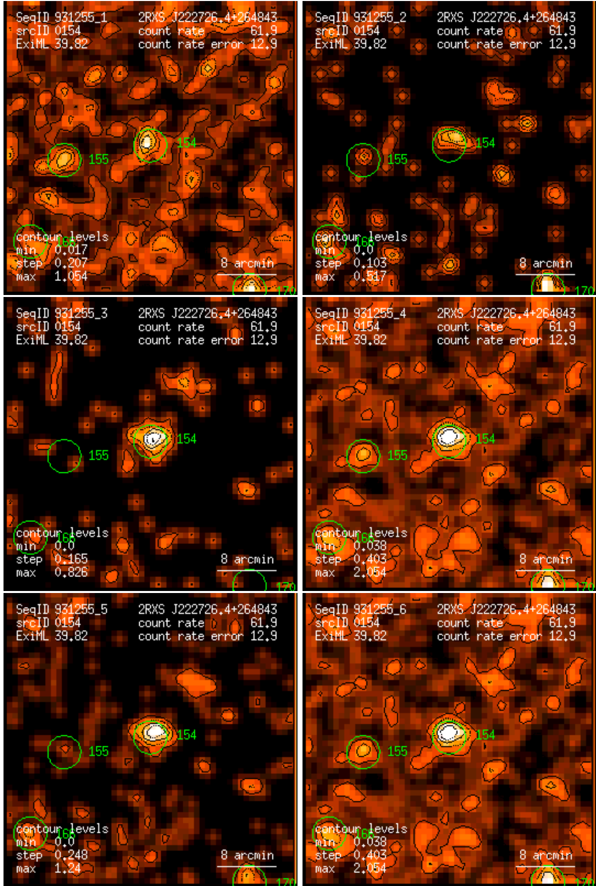
Figure 154: RASS 931255: detection 0154: band rate images, Gaussian filter: (1) PSPC channels 11 – 41, (2) 52 – 90, (3) 91 – 201, (4) 11 – 235, (5) 52 – 201, (6) 11 – 201. Broad band rates in counts/ks. Band rate contour levels in counts/ks/arcmin 2 .
