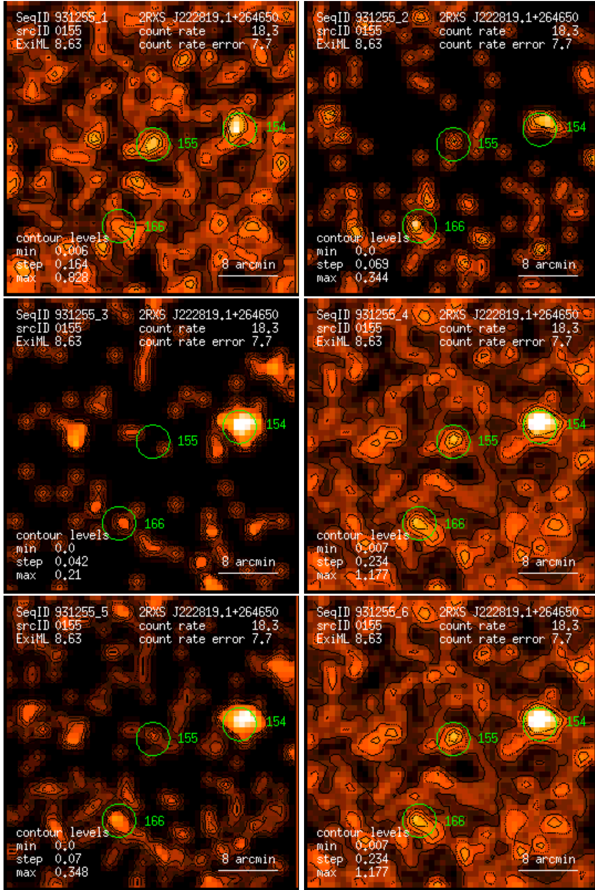
Figure 155: RASS 931255: detection 0155: band rate images, Gaussian filter: (1) PSPC channels 11 – 41, (2) 52 – 90, (3) 91 – 201, (4) 11 – 235, (5) 52 – 201, (6) 11 – 201. Broad band rates in counts/ks. Band rate contour levels in counts/ks/arcmin 2 .
