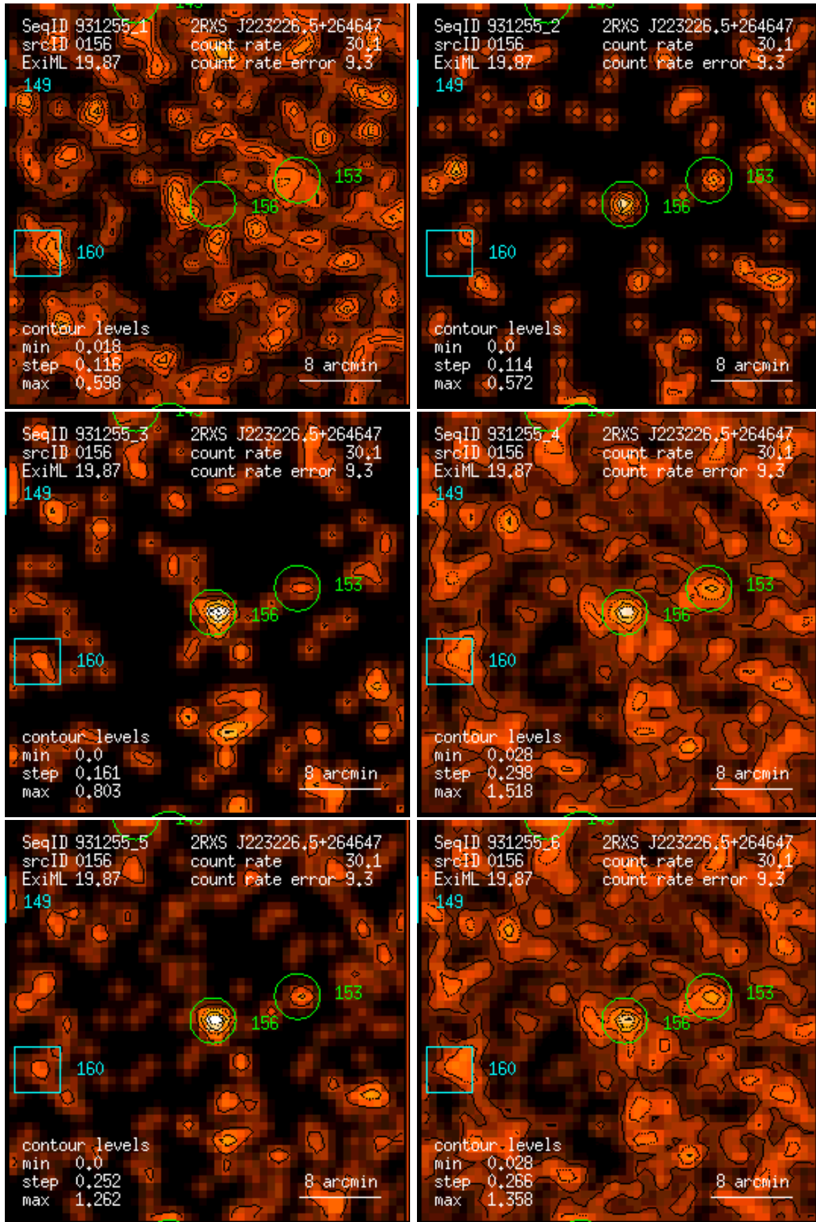
Figure 156: RASS 931255: detection 0156: band rate images, Gaussian filter: (1) PSPC channels 11 – 41, (2) 52 – 90, (3) 91 – 201, (4) 11 – 235, (5) 52 – 201, (6) 11 – 201. Broad band rates in counts/ks. Band rate contour levels in counts/ks/arcmin 2 .
