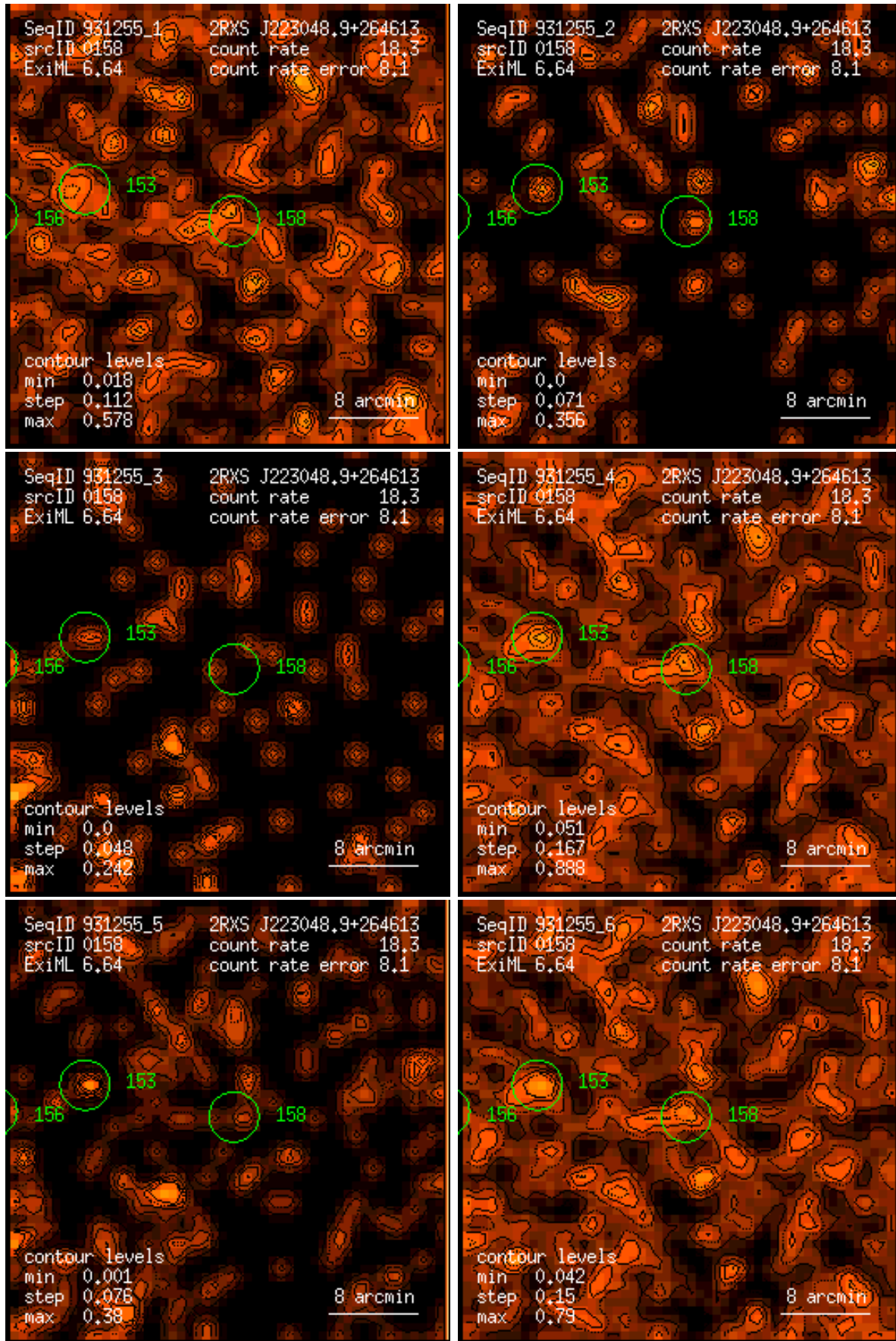
Figure 158: RASS 931255: detection 0158: band rate images, Gaussian filter: (1) PSPC channels 11 – 41, (2) 52 – 90, (3) 91 – 201, (4) 11 – 235, (5) 52 – 201, (6) 11 – 201. Broad band rates in counts/ks. Band rate contour levels in counts/ks/arcmin 2 .
