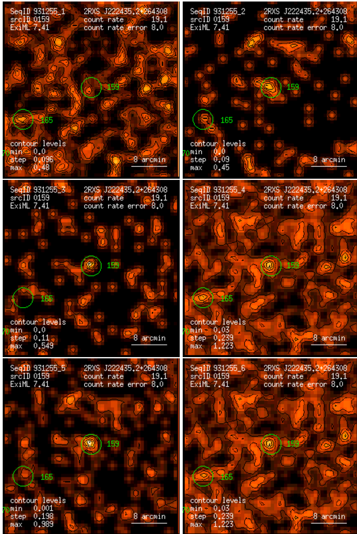
Figure 159: RASS 931255: detection 0159: band rate images, Gaussian filter: (1) PSPC channels 11 – 41, (2) 52 – 90, (3) 91 – 201, (4) 11 – 235, (5) 52 – 201, (6) 11 – 201. Broad band rates in counts/ks. Band rate contour levels in counts/ks/arcmin 2 .
