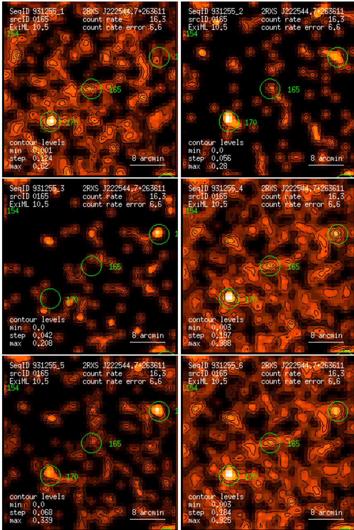
Figure 165: RASS 931255: detection 0165: band rate images, Gaussian filter: (1) PSPC channels 11 – 41, (2) 52 – 90, (3) 91 – 201, (4) 11 – 235, (5) 52 – 201, (6) 11 – 201. Broad band rates in counts/ks. Band rate contour levels in counts/ks/arcmin 2 .
