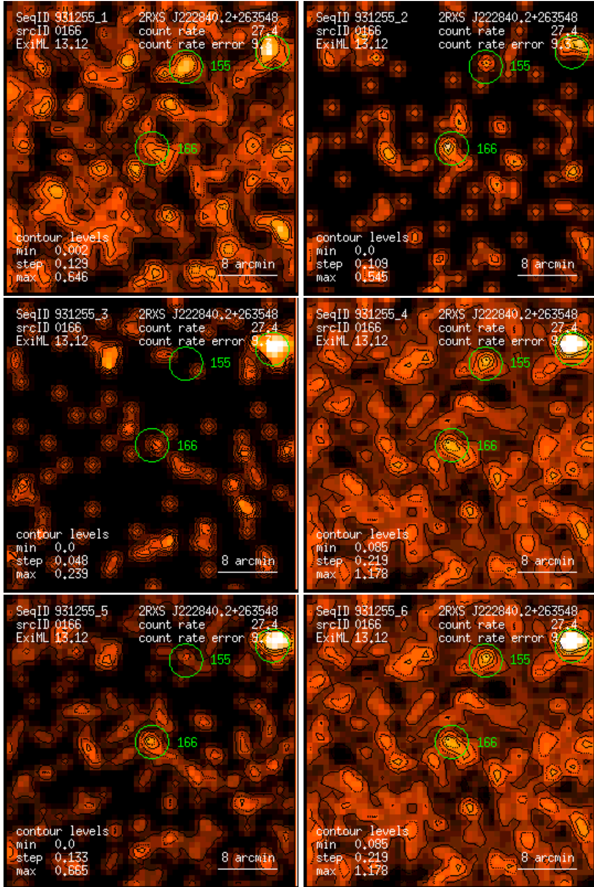
Figure 166: RASS 931255: detection 0166: band rate images, Gaussian filter: (1) PSPC channels 11 – 41, (2) 52 – 90, (3) 91 – 201, (4) 11 – 235, (5) 52 – 201, (6) 11 – 201. Broad band rates in counts/ks. Band rate contour levels in counts/ks/arcmin 2 .
