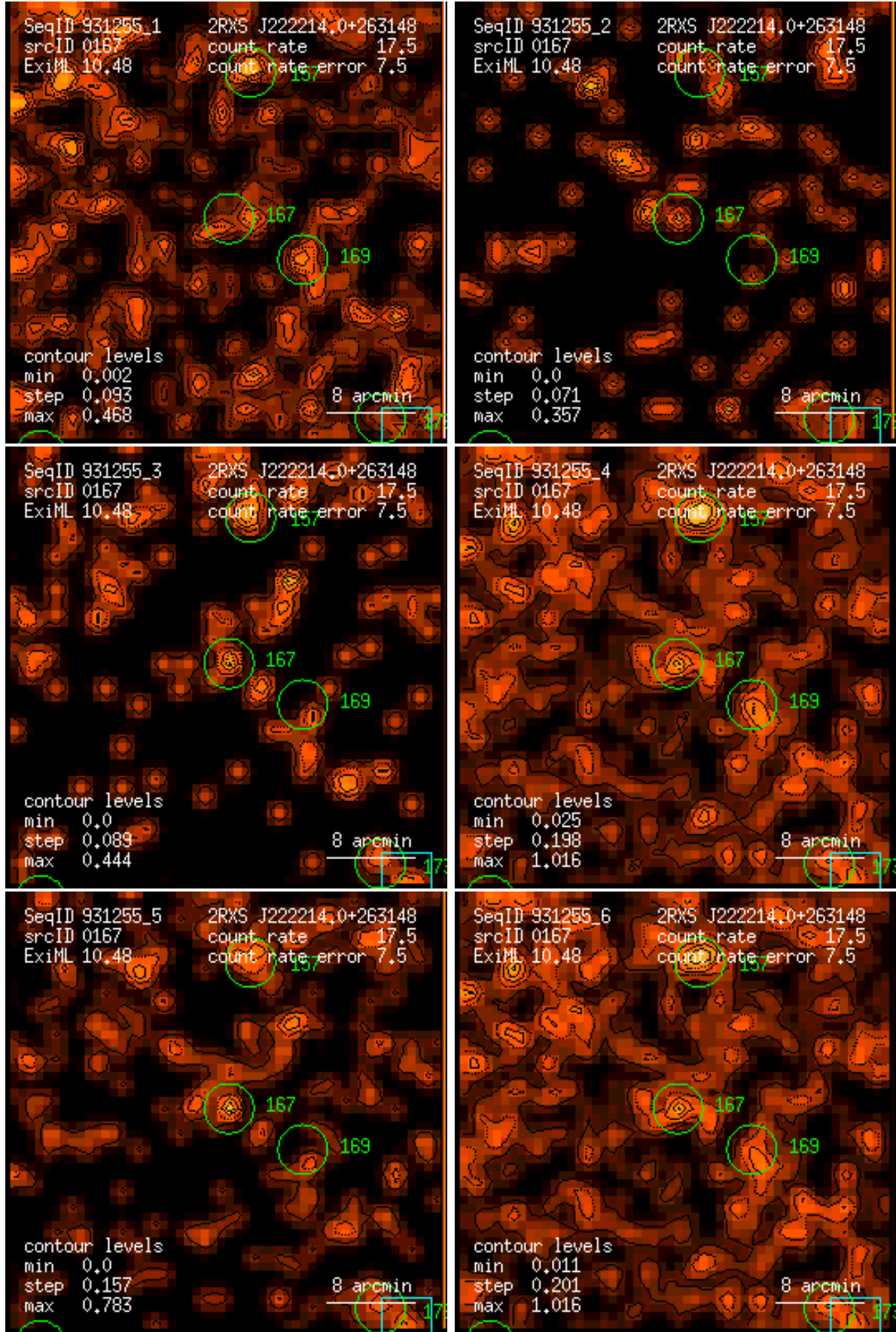
Figure 167: RASS 931255: detection 0167: band rate images, Gaussian filter: (1) PSPC channels 11 – 41, (2) 52 – 90, (3) 91 – 201, (4) 11 – 235, (5) 52 – 201, (6) 11 – 201. Broad band rates in counts/ks. Band rate contour levels in counts/ks/arcmin 2 .
