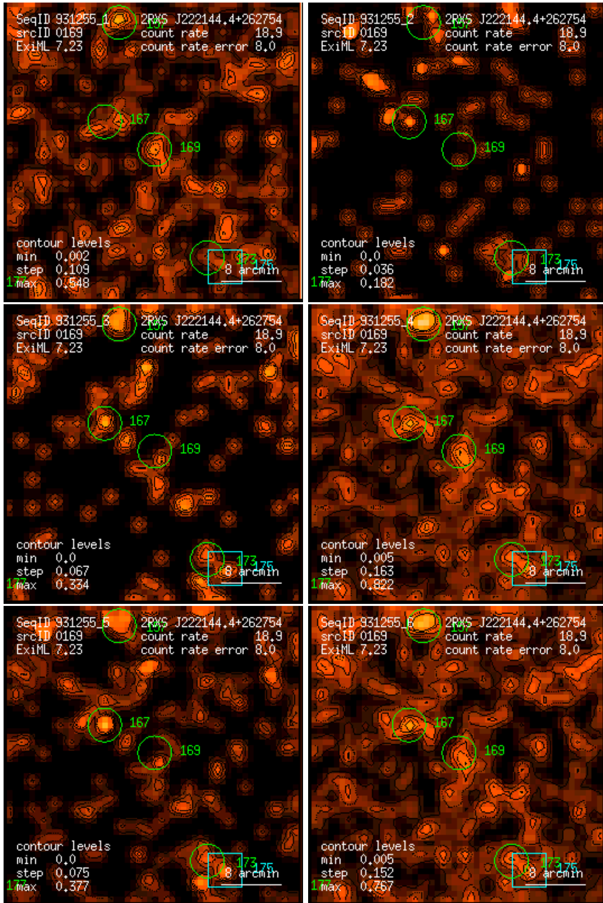
Figure 169: RASS 931255: detection 0169: band rate images, Gaussian filter: (1) PSPC channels 11 – 41, (2) 52 – 90, (3) 91 – 201, (4) 11 – 235, (5) 52 – 201, (6) 11 – 201. Broad band rates in counts/ks. Band rate contour levels in counts/ks/arcmin 2 .
