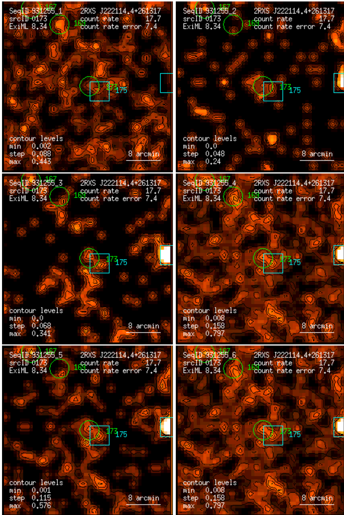
Figure 173: RASS 931255: detection 0173: band rate images, Gaussian filter: (1) PSPC channels 11 – 41, (2) 52 – 90, (3) 91 – 201, (4) 11 – 235, (5) 52 – 201, (6) 11 – 201. Broad band rates in counts/ks. Band rate contour levels in counts/ks/arcmin 2 .
