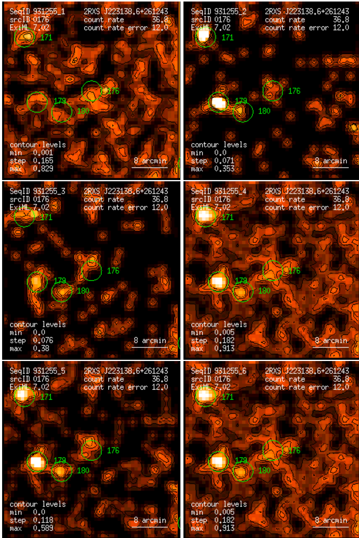
Figure 176: RASS 931255: detection 0176: band rate images, Gaussian filter: (1) PSPC channels 11 – 41, (2) 52 – 90, (3) 91 – 201, (4) 11 – 235, (5) 52 – 201, (6) 11 – 201. Broad band rates in counts/ks. Band rate contour levels in counts/ks/arcmin 2 .
