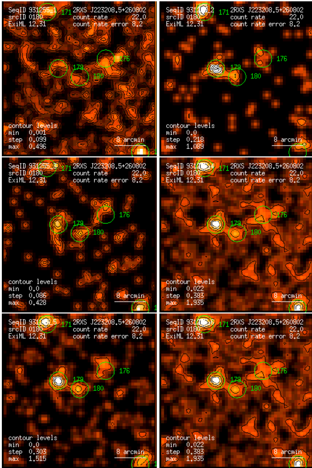
Figure 180: RASS 931255: detection 0180: band rate images, Gaussian filter: (1) PSPC channels 11 – 41, (2) 52 – 90, (3) 91 – 201, (4) 11 – 235, (5) 52 – 201, (6) 11 – 201. Broad band rates in counts/ks. Band rate contour levels in counts/ks/arcmin 2 .
