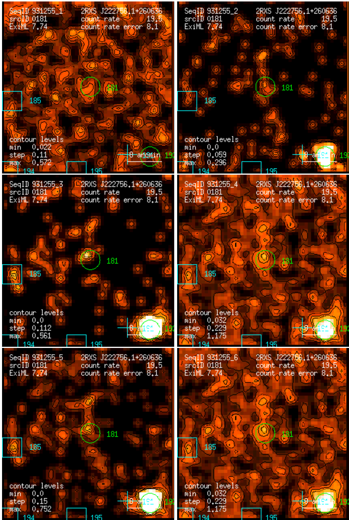
Figure 181: RASS 931255: detection 0181: band rate images, Gaussian filter: (1) PSPC channels 11 – 41, (2) 52 – 90, (3) 91 – 201, (4) 11 – 235, (5) 52 – 201, (6) 11 – 201. Broad band rates in counts/ks. Band rate contour levels in counts/ks/arcmin 2 .
