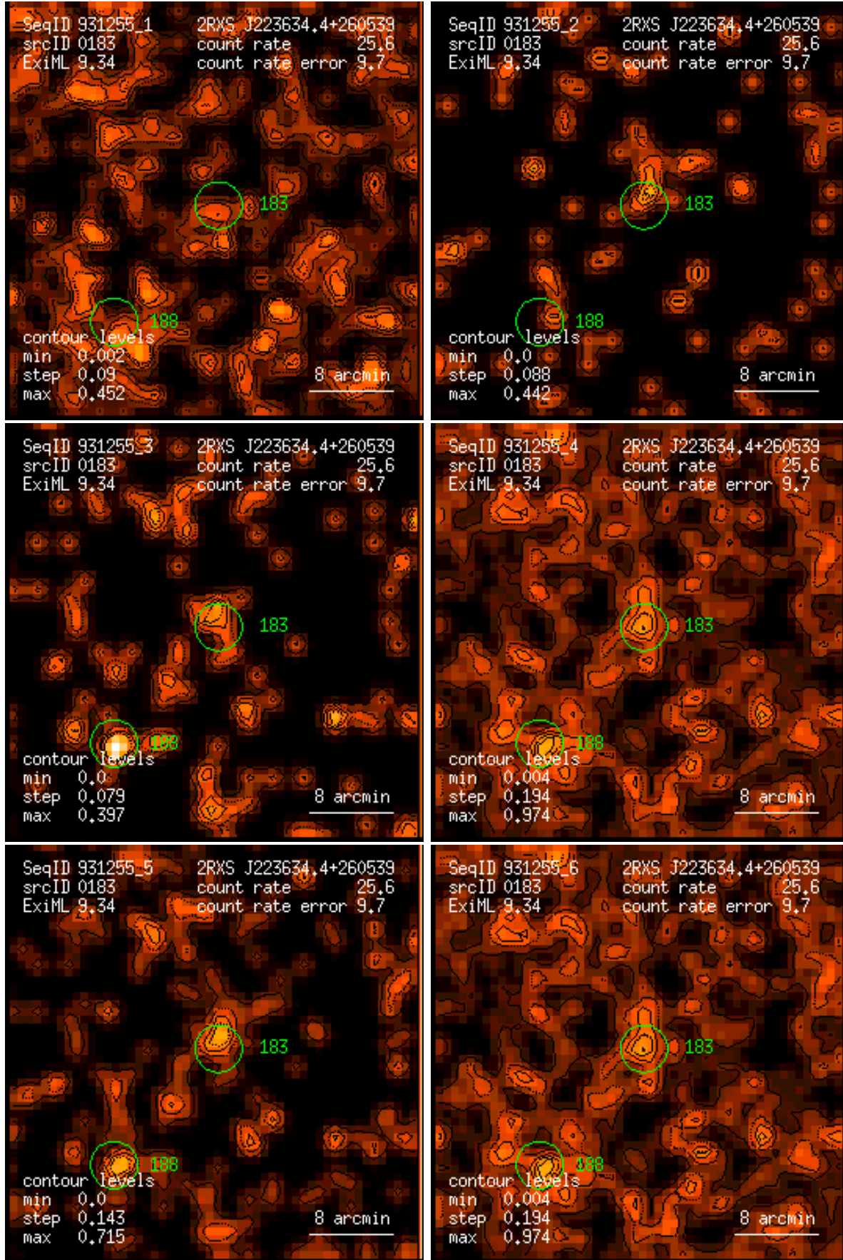
Figure 183: RASS 931255: detection 0183: band rate images, Gaussian filter: (1) PSPC channels 11 – 41, (2) 52 – 90, (3) 91 – 201, (4) 11 – 235, (5) 52 – 201, (6) 11 – 201. Broad band rates in counts/ks. Band rate contour levels in counts/ks/arcmin 2 .
