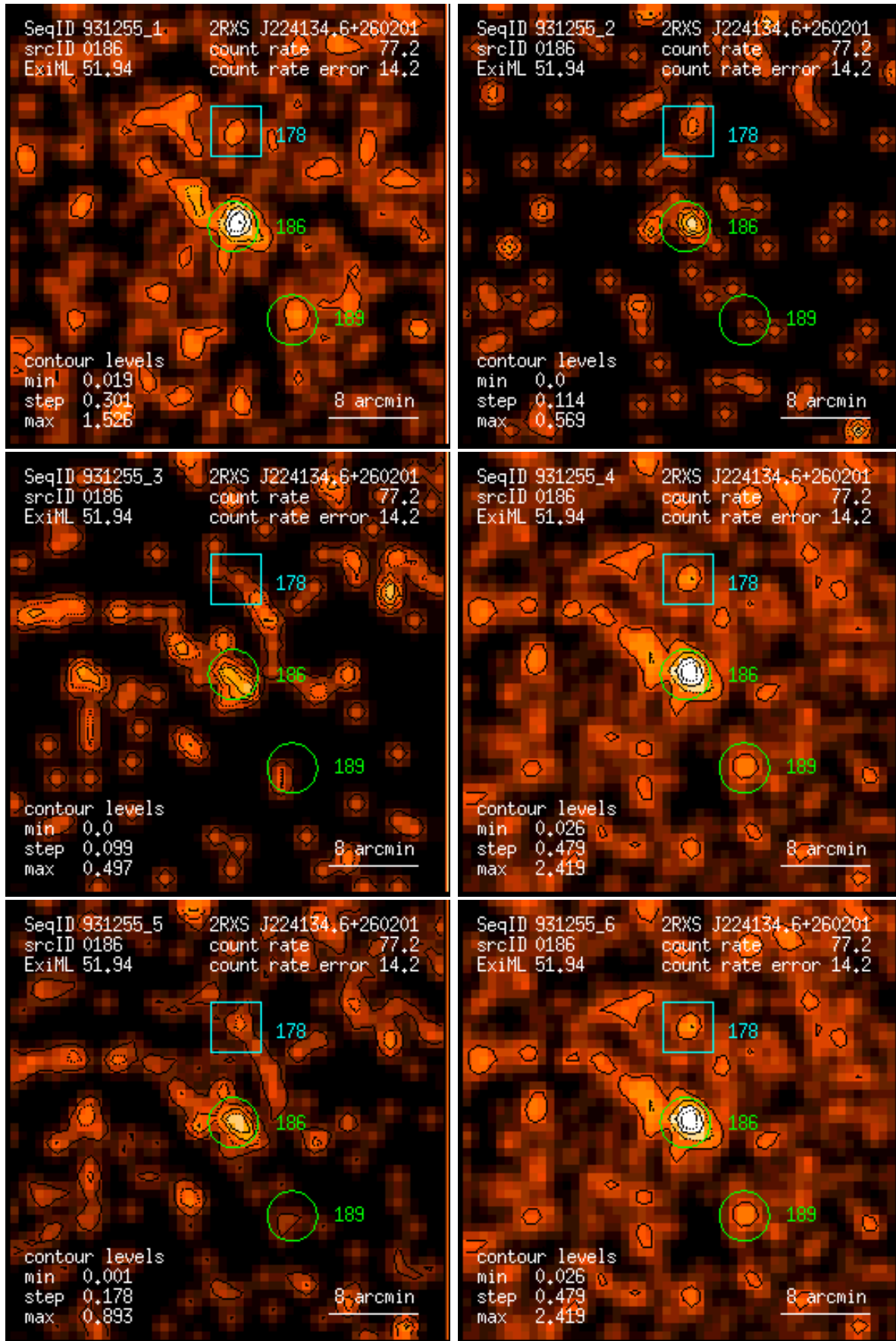
Figure 186: RASS 931255: detection 0186: band rate images, Gaussian filter: (1) PSPC channels 11 – 41, (2) 52 – 90, (3) 91 – 201, (4) 11 – 235, (5) 52 – 201, (6) 11 – 201. Broad band rates in counts/ks. Band rate contour levels in counts/ks/arcmin 2 .
