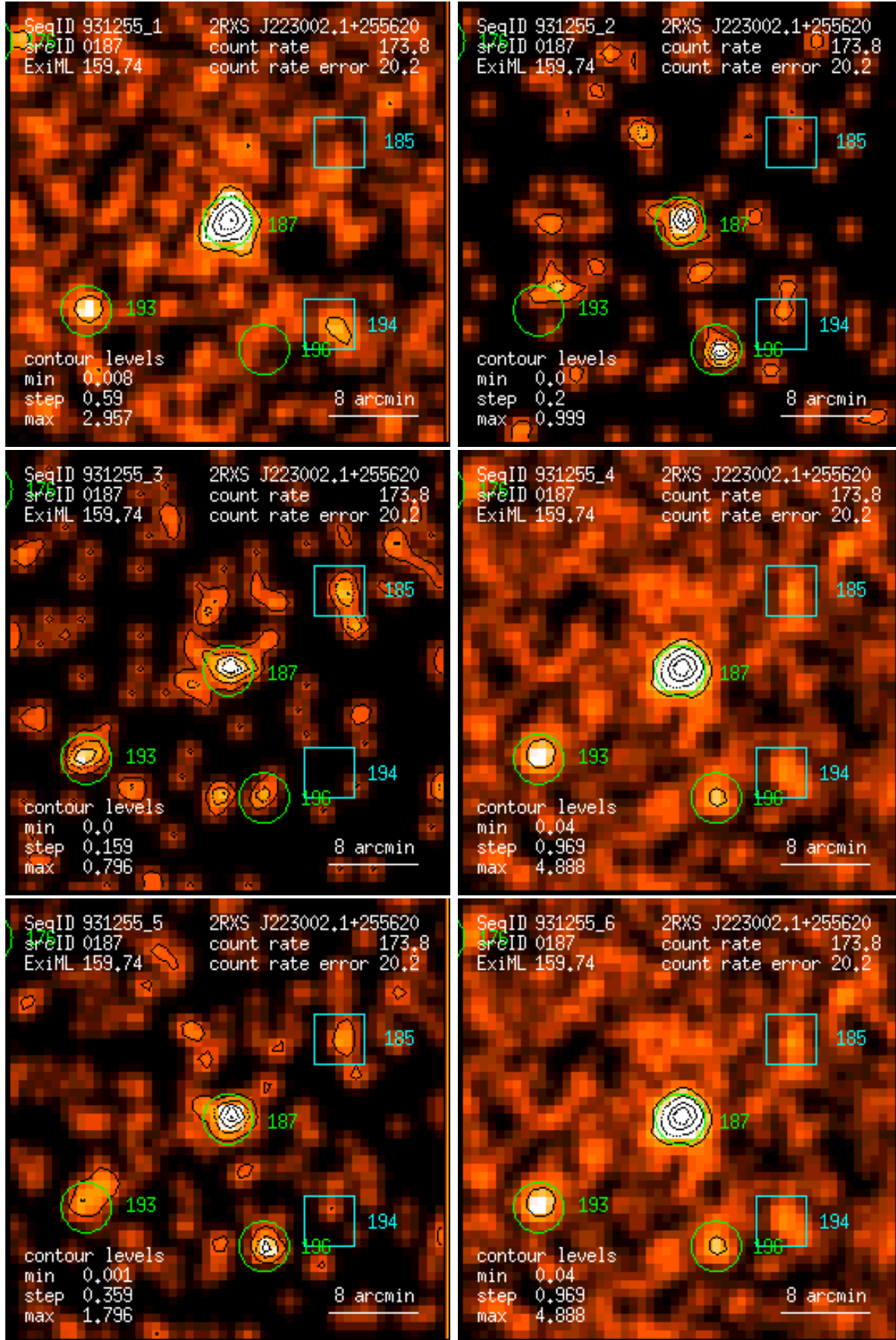
Figure 187: RASS 931255: detection 0187: band rate images, Gaussian filter: (1) PSPC channels 11 – 41, (2) 52 – 90, (3) 91 – 201, (4) 11 – 235, (5) 52 – 201, (6) 11 – 201. Broad band rates in counts/ks. Band rate contour levels in counts/ks/arcmin 2 .
