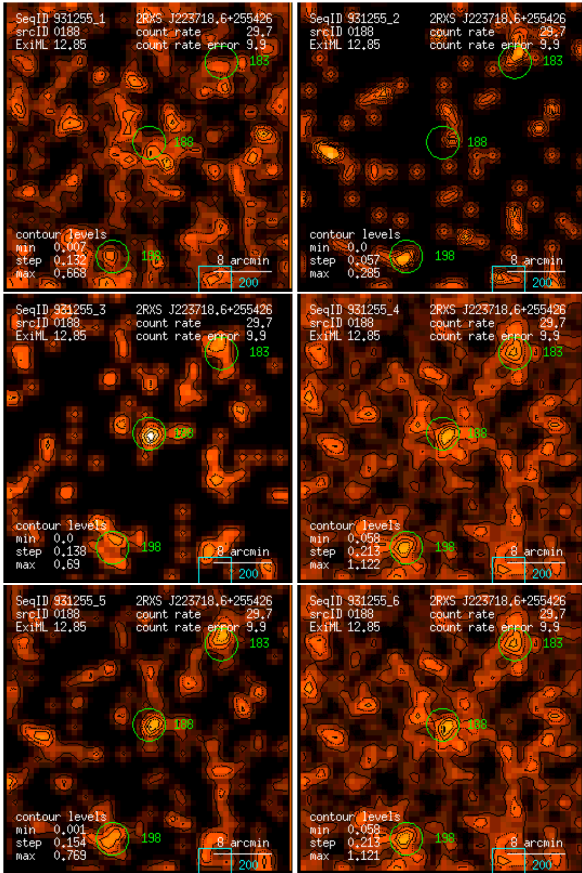
Figure 188: RASS 931255: detection 0188: band rate images, Gaussian filter: (1) PSPC channels 11 – 41, (2) 52 – 90, (3) 91 – 201, (4) 11 – 235, (5) 52 – 201, (6) 11 – 201. Broad band rates in counts/ks. Band rate contour levels in counts/ks/arcmin 2 .
