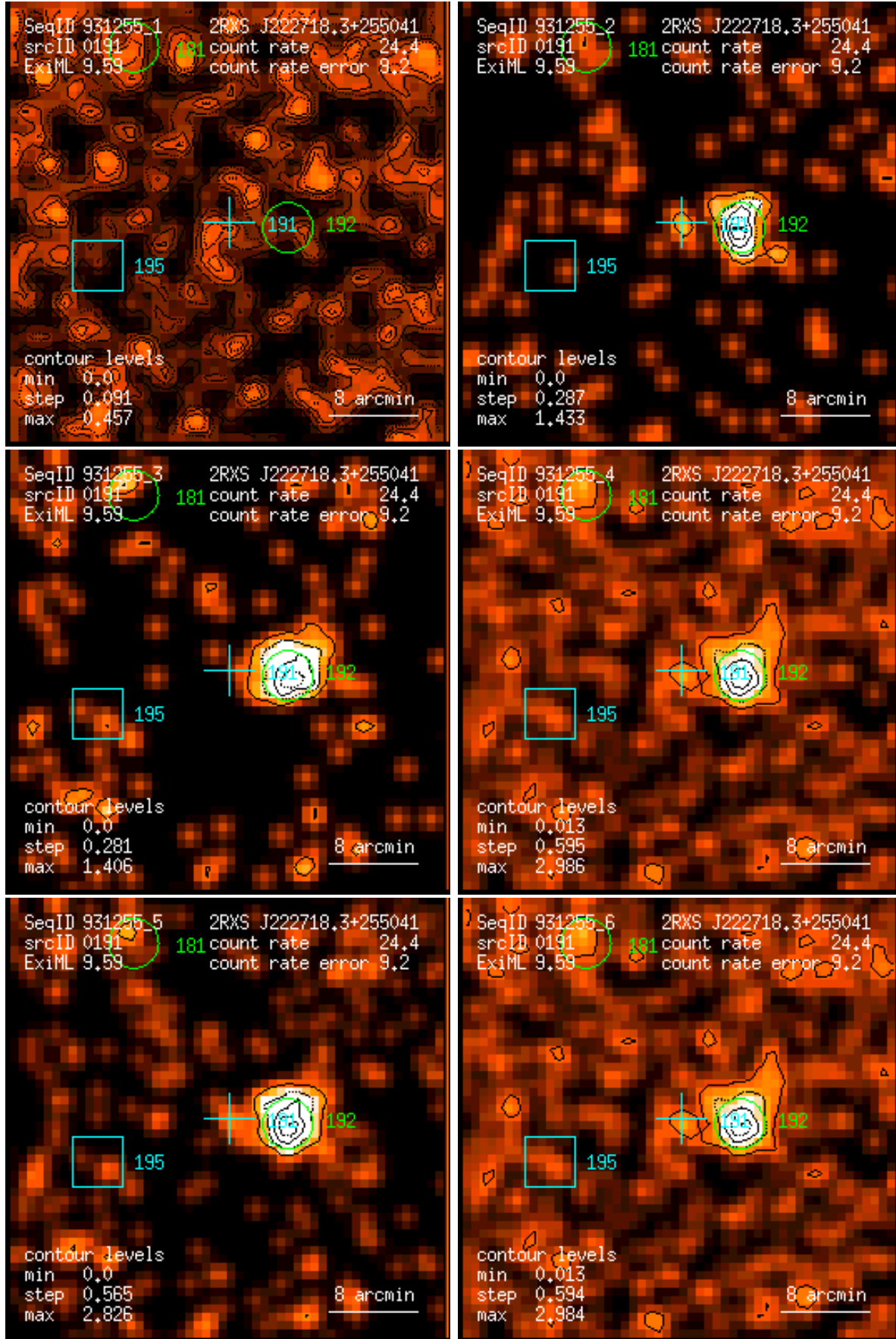
Figure 191: RASS 931255: detection 0191: band rate images, Gaussian filter: (1) PSPC channels 11 – 41, (2) 52 – 90, (3) 91 – 201, (4) 11 – 235, (5) 52 – 201, (6) 11 – 201. Broad band rates in counts/ks. Band rate contour levels in counts/ks/arcmin 2 .
