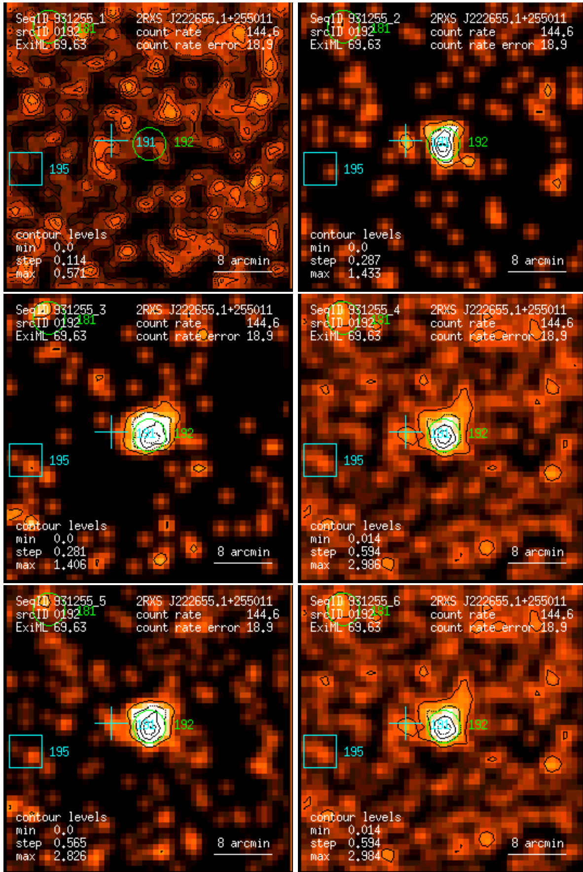
Figure 192: RASS 931255: detection 0192: band rate images, Gaussian filter: (1) PSPC channels 11 – 41, (2) 52 – 90, (3) 91 – 201, (4) 11 – 235, (5) 52 – 201, (6) 11 – 201. Broad band rates in counts/ks. Band rate contour levels in counts/ks/arcmin 2 .
