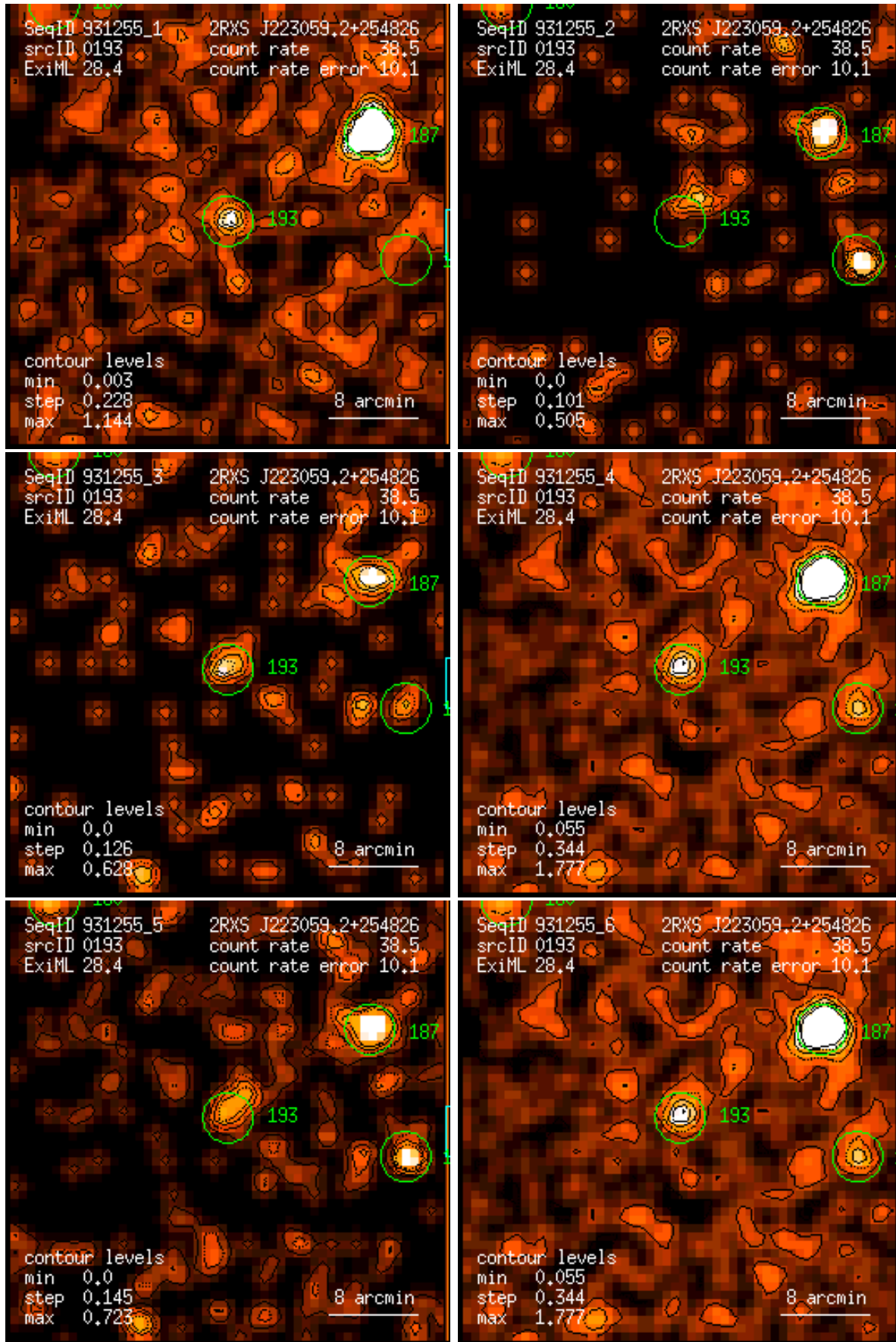
Figure 193: RASS 931255: detection 0193: band rate images, Gaussian filter: (1) PSPC channels 11 – 41, (2) 52 – 90, (3) 91 – 201, (4) 11 – 235, (5) 52 – 201, (6) 11 – 201. Broad band rates in counts/ks. Band rate contour levels in counts/ks/arcmin 2 .
