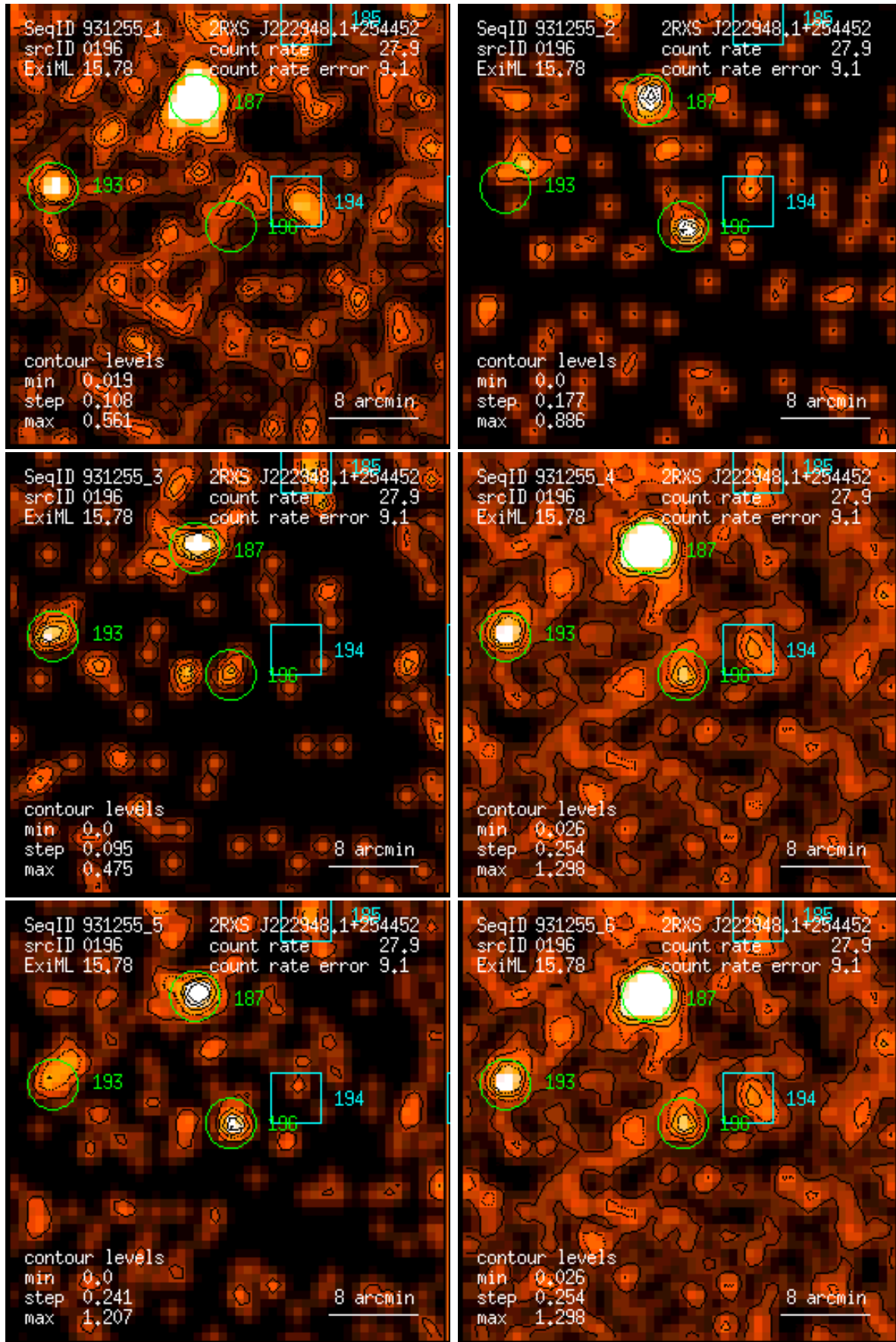
Figure 196: RASS 931255: detection 0196: band rate images, Gaussian filter: (1) PSPC channels 11 – 41, (2) 52 – 90, (3) 91 – 201, (4) 11 – 235, (5) 52 – 201, (6) 11 – 201. Broad band rates in counts/ks. Band rate contour levels in counts/ks/arcmin 2 .
