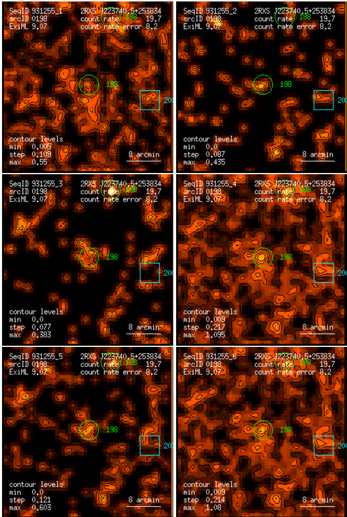
Figure 198: RASS 931255: detection 0198: band rate images, Gaussian filter: (1) PSPC channels 11 – 41, (2) 52 – 90, (3) 91 – 201, (4) 11 – 235, (5) 52 – 201, (6) 11 – 201. Broad band rates in counts/ks. Band rate contour levels in counts/ks/arcmin 2 .
