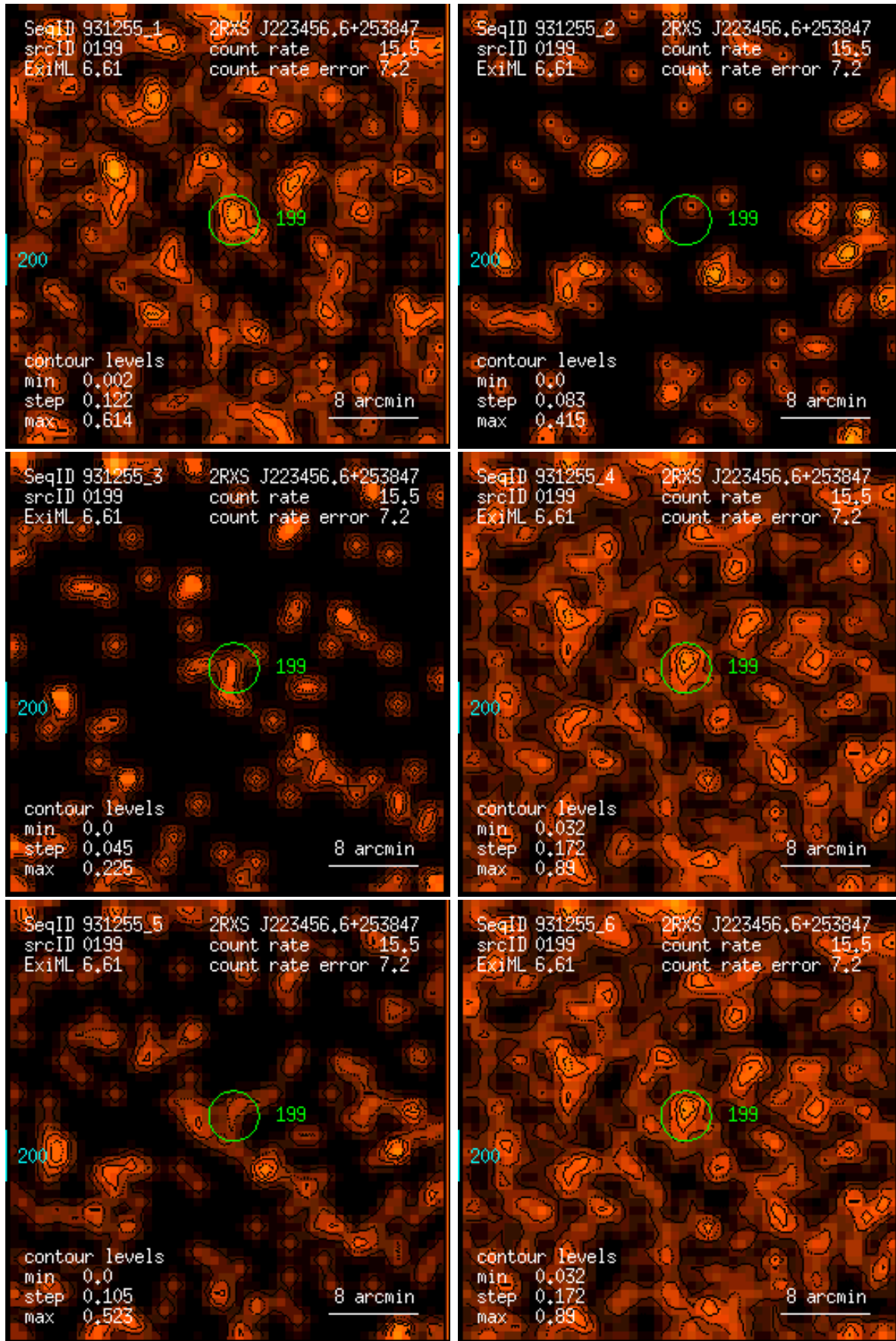
Figure 199: RASS 931255: detection 0199: band rate images, Gaussian filter: (1) PSPC channels 11 – 41, (2) 52 – 90, (3) 91 – 201, (4) 11 – 235, (5) 52 – 201, (6) 11 – 201. Broad band rates in counts/ks. Band rate contour levels in counts/ks/arcmin 2 .
