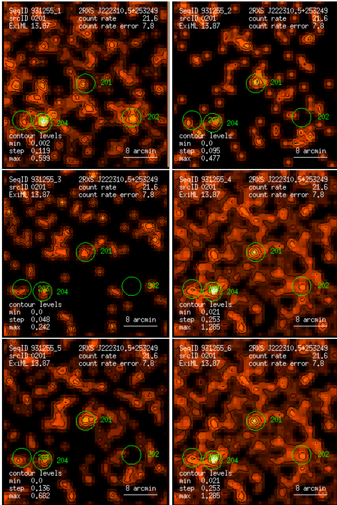
Figure 201: RASS 931255: detection 0201: band rate images, Gaussian filter: (1) PSPC channels 11 – 41, (2) 52 – 90, (3) 91 – 201, (4) 11 – 235, (5) 52 – 201, (6) 11 – 201. Broad band rates in counts/ks. Band rate contour levels in counts/ks/arcmin 2 .
