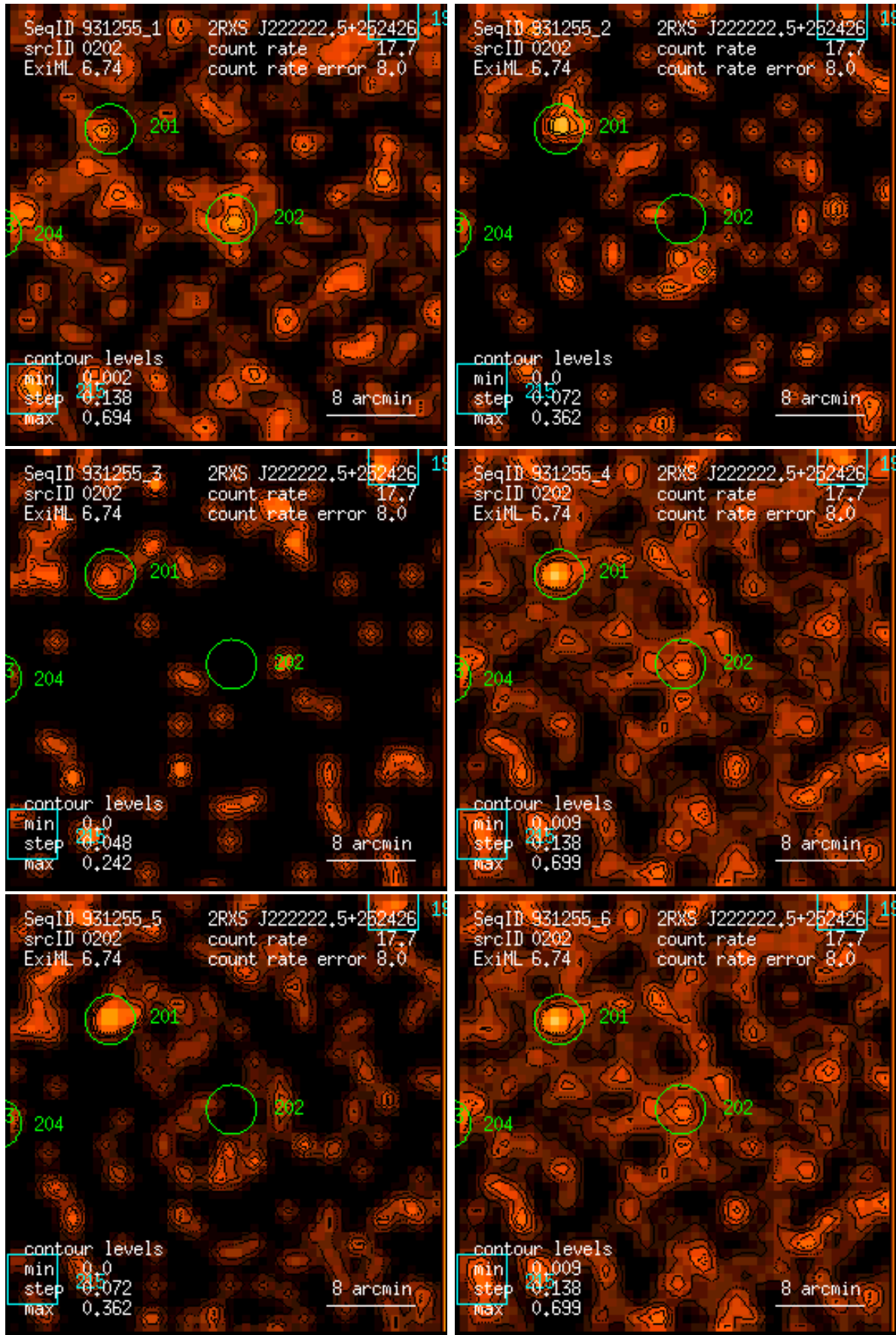
Figure 202: RASS 931255: detection 0202: band rate images, Gaussian filter: (1) PSPC channels 11 – 41, (2) 52 – 90, (3) 91 – 201, (4) 11 – 235, (5) 52 – 201, (6) 11 – 201. Broad band rates in counts/ks. Band rate contour levels in counts/ks/arcmin 2 .
