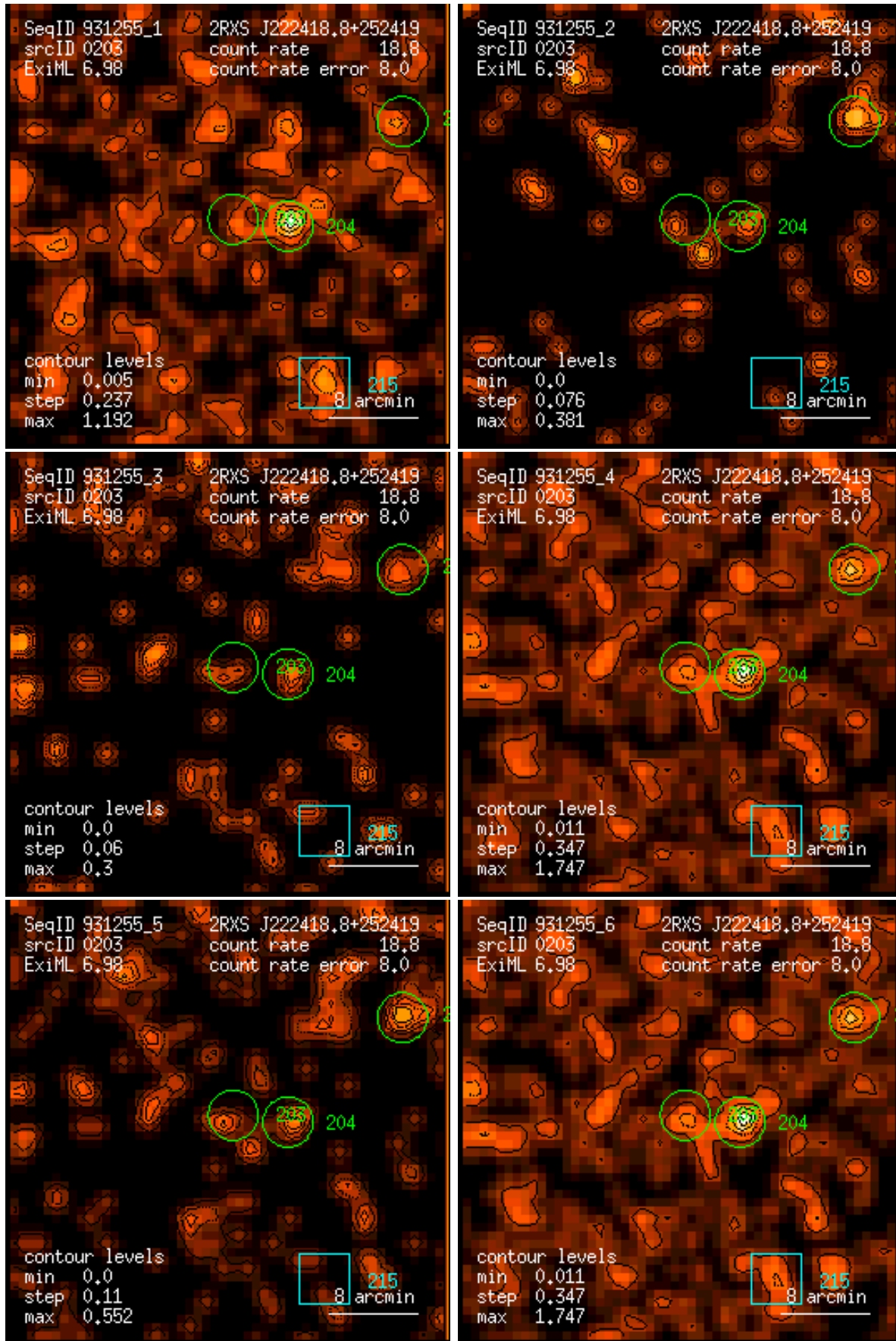
Figure 203: RASS 931255: detection 0203: band rate images, Gaussian filter: (1) PSPC channels 11 – 41, (2) 52 – 90, (3) 91 – 201, (4) 11 – 235, (5) 52 – 201, (6) 11 – 201. Broad band rates in counts/ks. Band rate contour levels in counts/ks/arcmin 2 .
