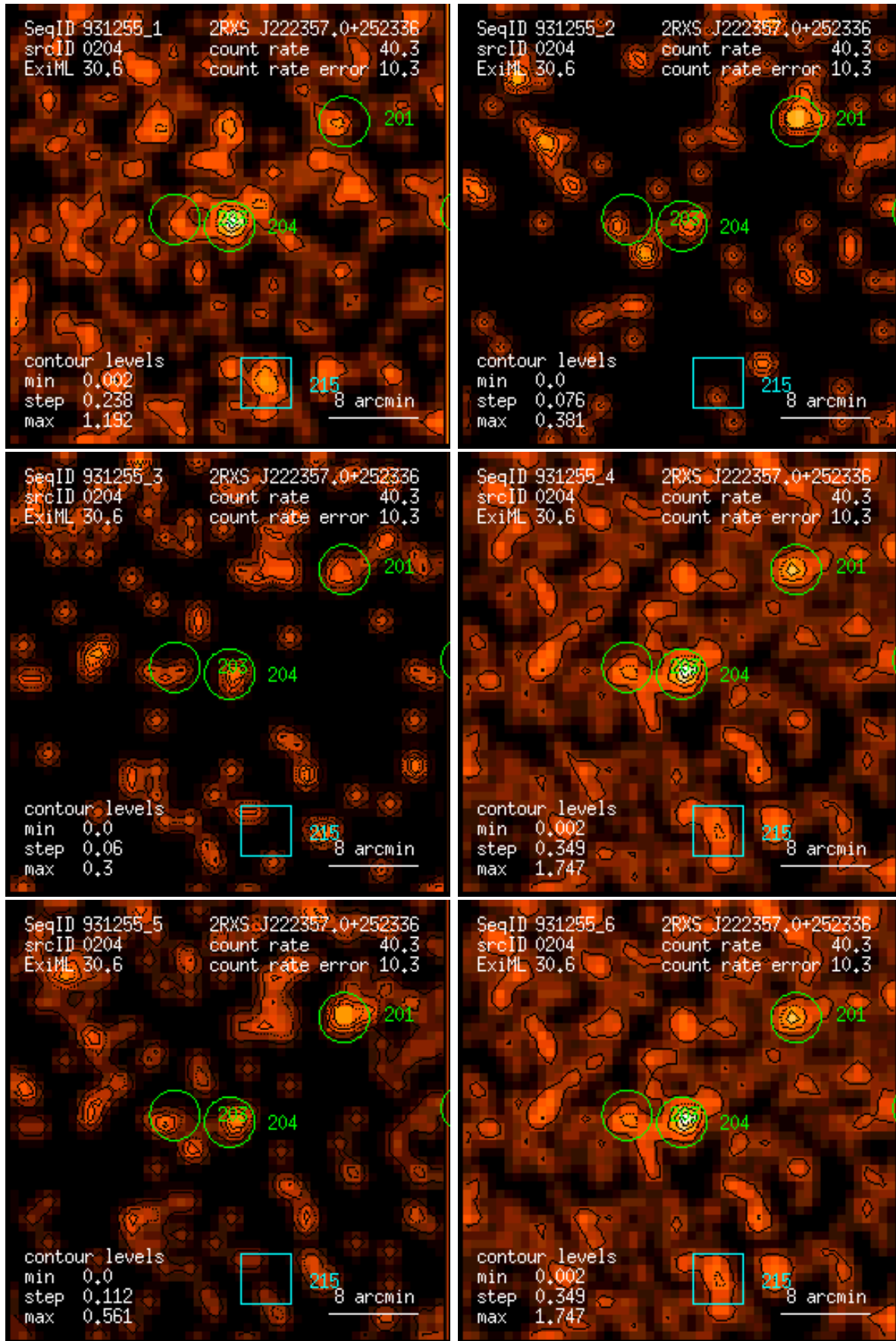
Figure 204: RASS 931255: detection 0204: band rate images, Gaussian filter: (1) PSPC channels 11 – 41, (2) 52 – 90, (3) 91 – 201, (4) 11 – 235, (5) 52 – 201, (6) 11 – 201. Broad band rates in counts/ks. Band rate contour levels in counts/ks/arcmin 2 .
