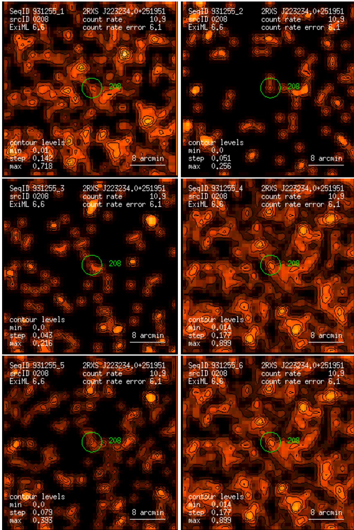
Figure 208: RASS 931255: detection 0208: band rate images, Gaussian filter: (1) PSPC channels 11 – 41, (2) 52 – 90, (3) 91 – 201, (4) 11 – 235, (5) 52 – 201, (6) 11 – 201. Broad band rates in counts/ks. Band rate contour levels in counts/ks/arcmin 2 .
