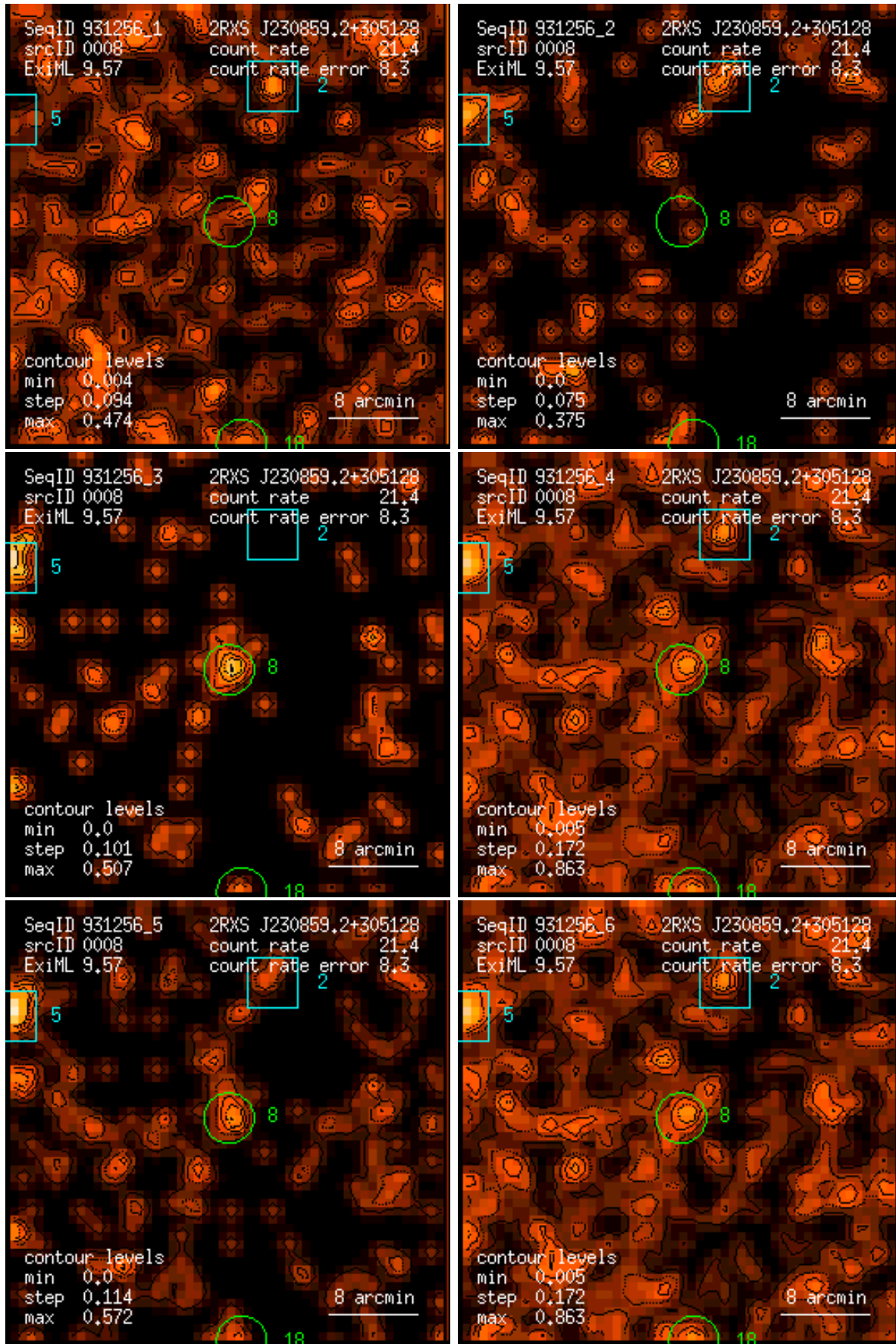
Figure 8: RASS 931256: detection 0008: band rate images, Gaussian filter: (1) PSPC channels 11 – 41, (2) 52 – 90, (3) 91 – 201, (4) 11 – 235, (5) 52 – 201, (6) 11 – 201. Broad band rates in counts/ks. Band rate contour levels in counts/ks/arcmin 2 .
