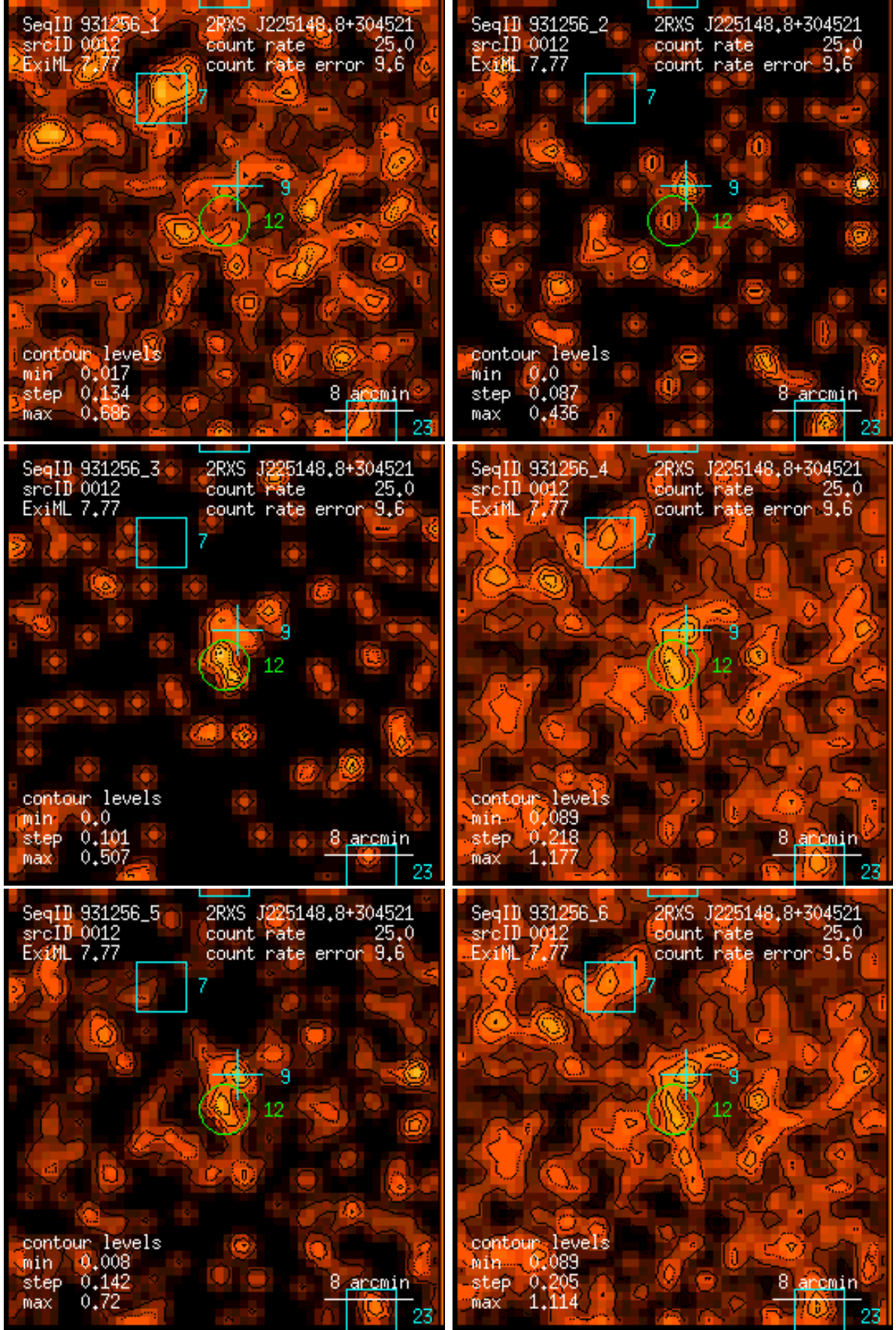
Figure 12: RASS 931256: detection 0012: band rate images, Gaussian filter: (1) PSPC channels 11 – 41, (2) 52 – 90, (3) 91 – 201, (4) 11 – 235, (5) 52 – 201, (6) 11 – 201. Broad band rates in counts/ks. Band rate contour levels in counts/ks/arcmin 2 .
