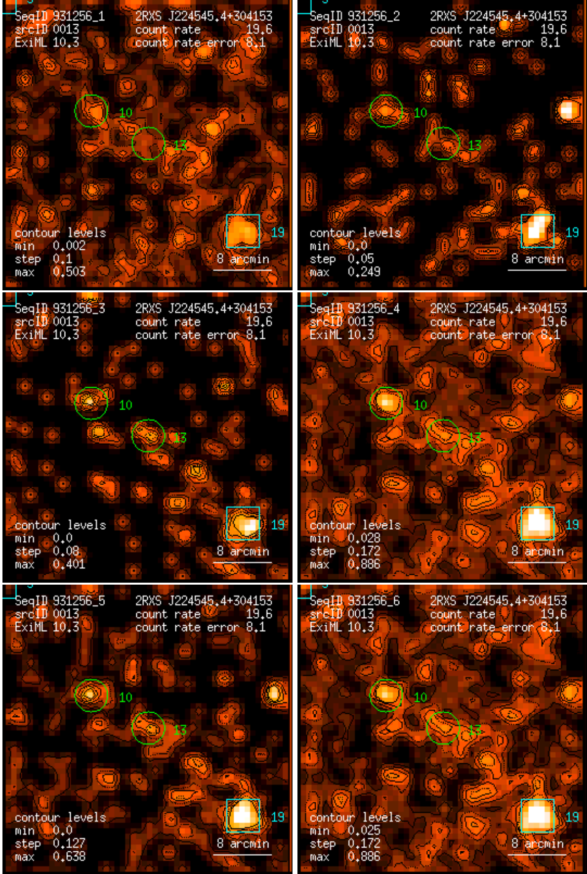
Figure 13: RASS 931256: detection 0013: band rate images, Gaussian filter: (1) PSPC channels 11 – 41, (2) 52 – 90, (3) 91 – 201, (4) 11 – 235, (5) 52 – 201, (6) 11 – 201. Broad band rates in counts/ks. Band rate contour levels in counts/ks/arcmin 2 .
