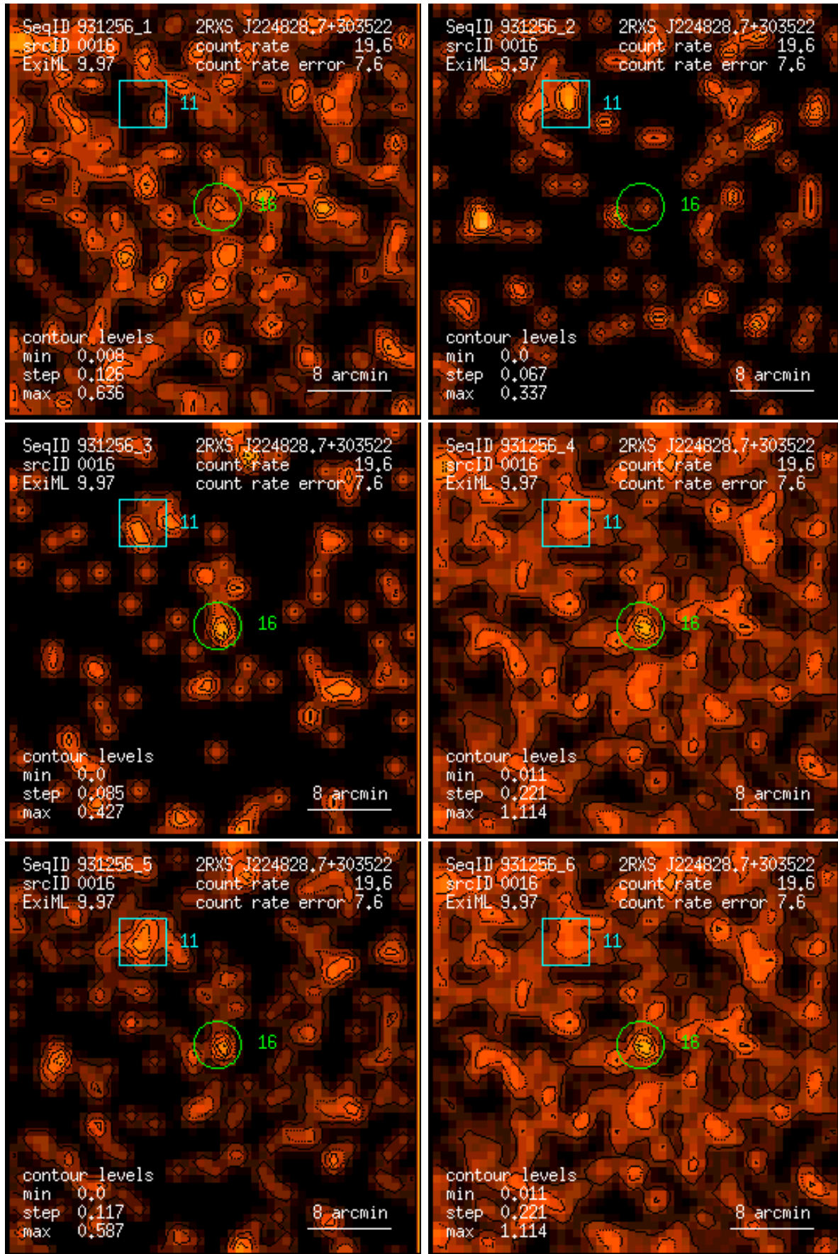
Figure 16: RASS 931256: detection 0016: band rate images, Gaussian filter: (1) PSPC channels 11 – 41, (2) 52 – 90, (3) 91 – 201, (4) 11 – 235, (5) 52 – 201, (6) 11 – 201. Broad band rates in counts/ks. Band rate contour levels in counts/ks/arcmin 2 .
