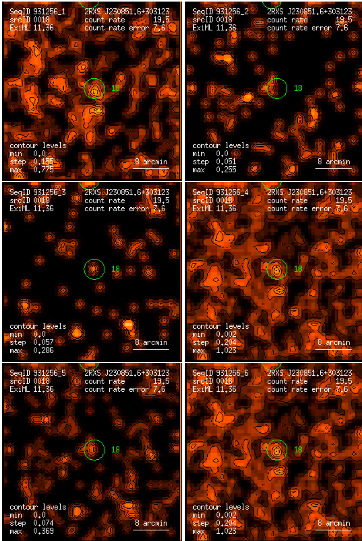
Figure 18: RASS 931256: detection 0018: band rate images, Gaussian filter: (1) PSPC channels 11 – 41, (2) 52 – 90, (3) 91 – 201, (4) 11 – 235, (5) 52 – 201, (6) 11 – 201. Broad band rates in counts/ks. Band rate contour levels in counts/ks/arcmin 2 .
