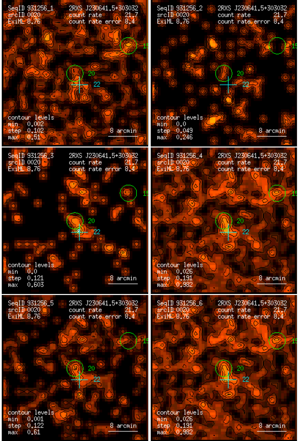
Figure 20: RASS 931256: detection 0020: band rate images, Gaussian filter: (1) PSPC channels 11 – 41, (2) 52 – 90, (3) 91 – 201, (4) 11 – 235, (5) 52 – 201, (6) 11 – 201. Broad band rates in counts/ks. Band rate contour levels in counts/ks/arcmin 2 .
