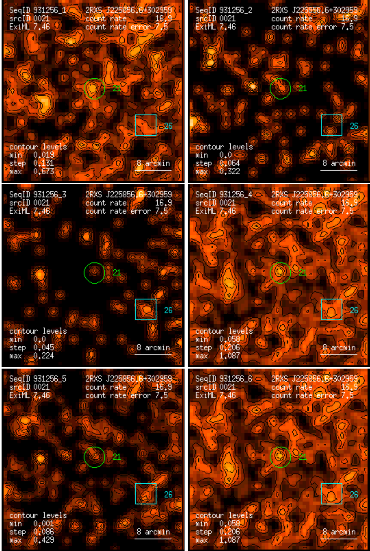
Figure 21: RASS 931256: detection 0021: band rate images, Gaussian filter: (1) PSPC channels 11 – 41, (2) 52 – 90, (3) 91 – 201, (4) 11 – 235, (5) 52 – 201, (6) 11 – 201. Broad band rates in counts/ks. Band rate contour levels in counts/ks/arcmin 2 .
