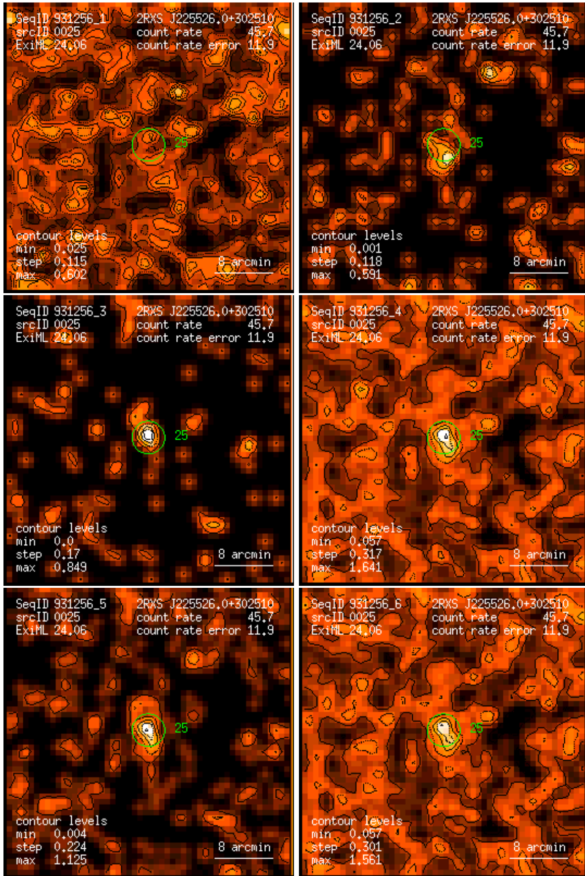
Figure 25: RASS 931256: detection 0025: band rate images, Gaussian filter: (1) PSPC channels 11 – 41, (2) 52 – 90, (3) 91 – 201, (4) 11 – 235, (5) 52 – 201, (6) 11 – 201. Broad band rates in counts/ks. Band rate contour levels in counts/ks/arcmin 2 .
