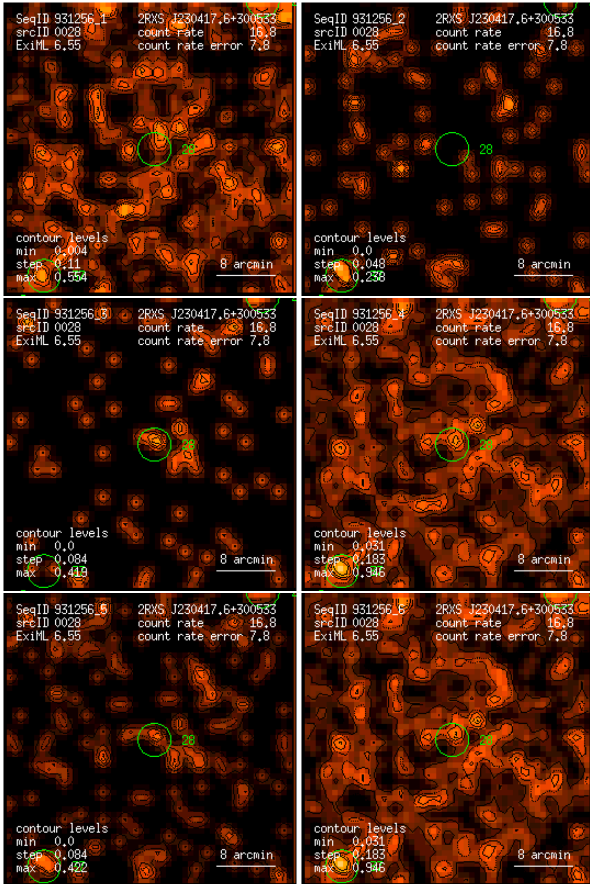
Figure 28: RASS 931256: detection 0028: band rate images, Gaussian filter: (1) PSPC channels 11 – 41, (2) 52 – 90, (3) 91 – 201, (4) 11 – 235, (5) 52 – 201, (6) 11 – 201. Broad band rates in counts/ks. Band rate contour levels in counts/ks/arcmin 2 .
