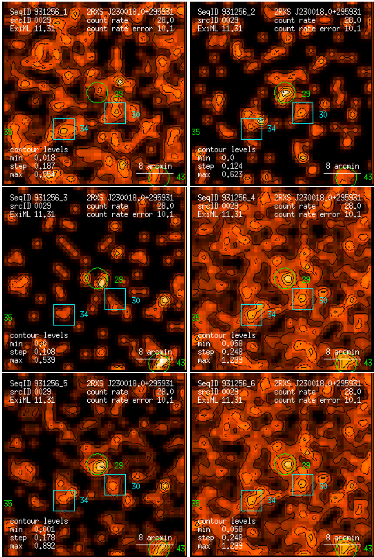
Figure 29: RASS 931256: detection 0029: band rate images, Gaussian filter: (1) PSPC channels 11 – 41, (2) 52 – 90, (3) 91 – 201, (4) 11 – 235, (5) 52 – 201, (6) 11 – 201. Broad band rates in counts/ks. Band rate contour levels in counts/ks/arcmin 2 .
