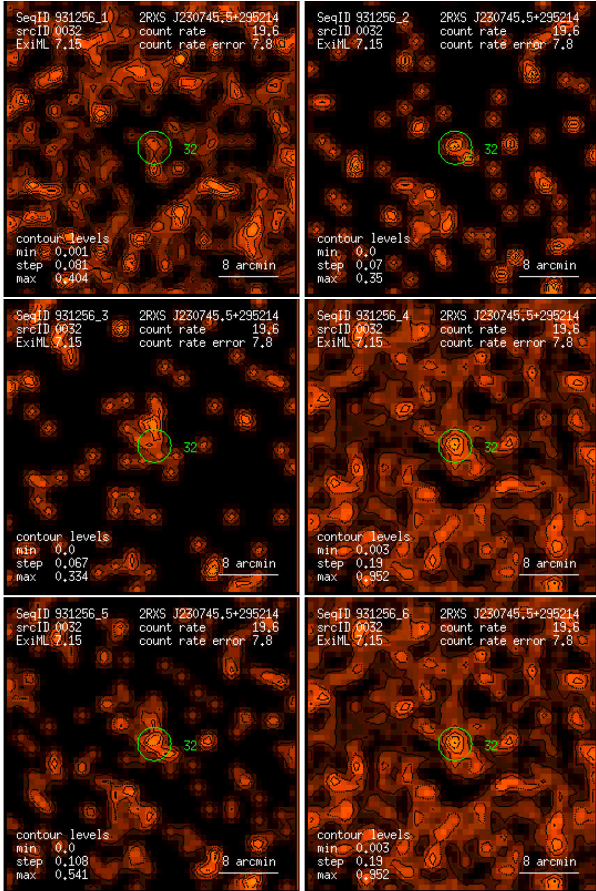
Figure 32: RASS 931256: detection 0032: band rate images, Gaussian filter: (1) PSPC channels 11 – 41, (2) 52 – 90, (3) 91 – 201, (4) 11 – 235, (5) 52 – 201, (6) 11 – 201. Broad band rates in counts/ks. Band rate contour levels in counts/ks/arcmin 2 .
