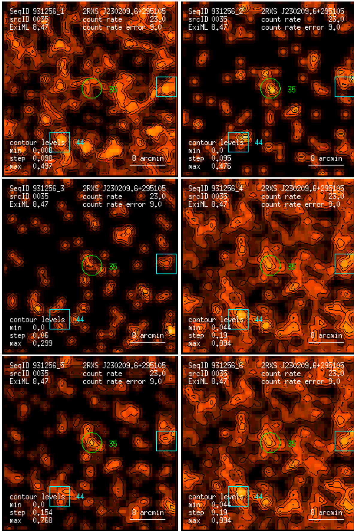
Figure 35: RASS 931256: detection 0035: band rate images, Gaussian filter: (1) PSPC channels 11 – 41, (2) 52 – 90, (3) 91 – 201, (4) 11 – 235, (5) 52 – 201, (6) 11 – 201. Broad band rates in counts/ks. Band rate contour levels in counts/ks/arcmin 2 .
