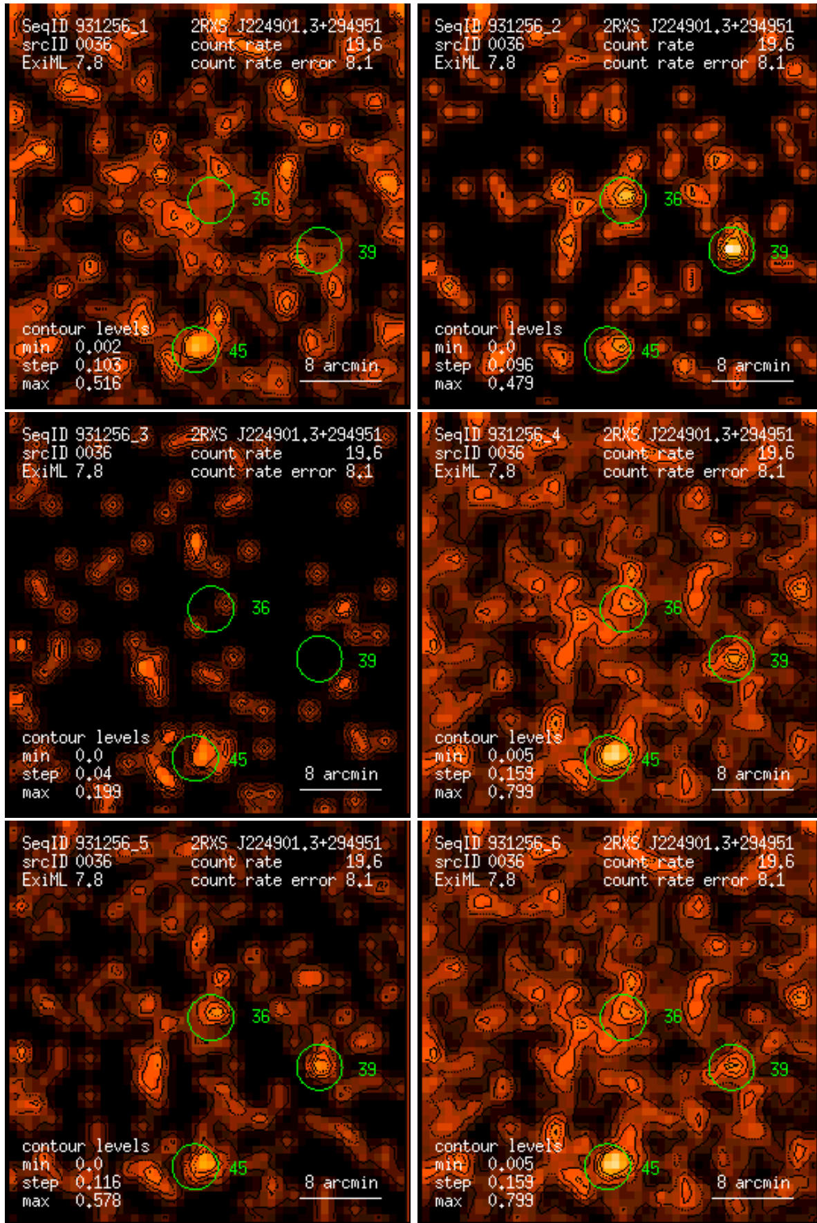
Figure 36: RASS 931256: detection 0036: band rate images, Gaussian filter: (1) PSPC channels 11 – 41, (2) 52 – 90, (3) 91 – 201, (4) 11 – 235, (5) 52 – 201, (6) 11 – 201. Broad band rates in counts/ks. Band rate contour levels in counts/ks/arcmin 2 .
