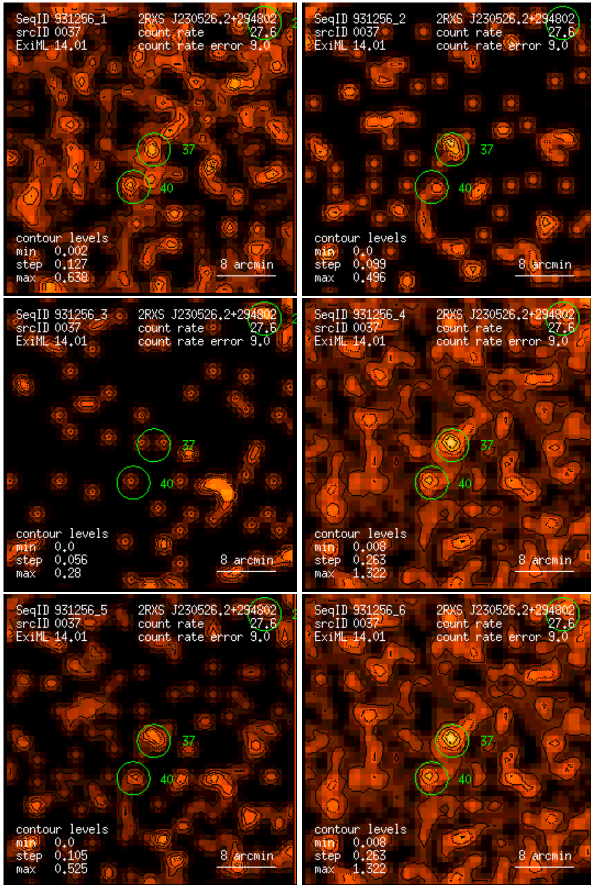
Figure 37: RASS 931256: detection 0037: band rate images, Gaussian filter: (1) PSPC channels 11 – 41, (2) 52 – 90, (3) 91 – 201, (4) 11 – 235, (5) 52 – 201, (6) 11 – 201. Broad band rates in counts/ks. Band rate contour levels in counts/ks/arcmin 2 .
