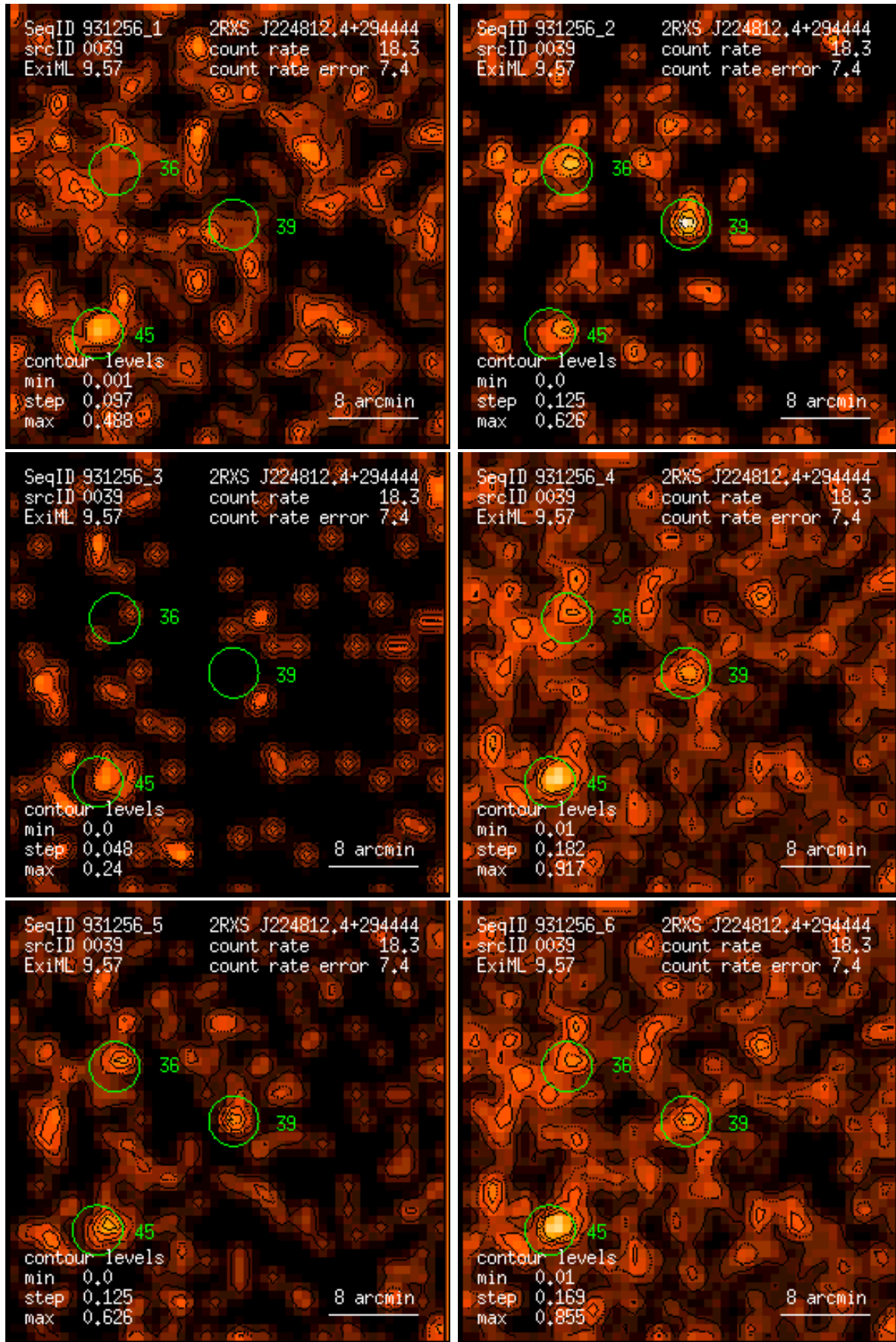
Figure 39: RASS 931256: detection 0039: band rate images, Gaussian filter: (1) PSPC channels 11 – 41, (2) 52 – 90, (3) 91 – 201, (4) 11 – 235, (5) 52 – 201, (6) 11 – 201. Broad band rates in counts/ks. Band rate contour levels in counts/ks/arcmin 2 .
