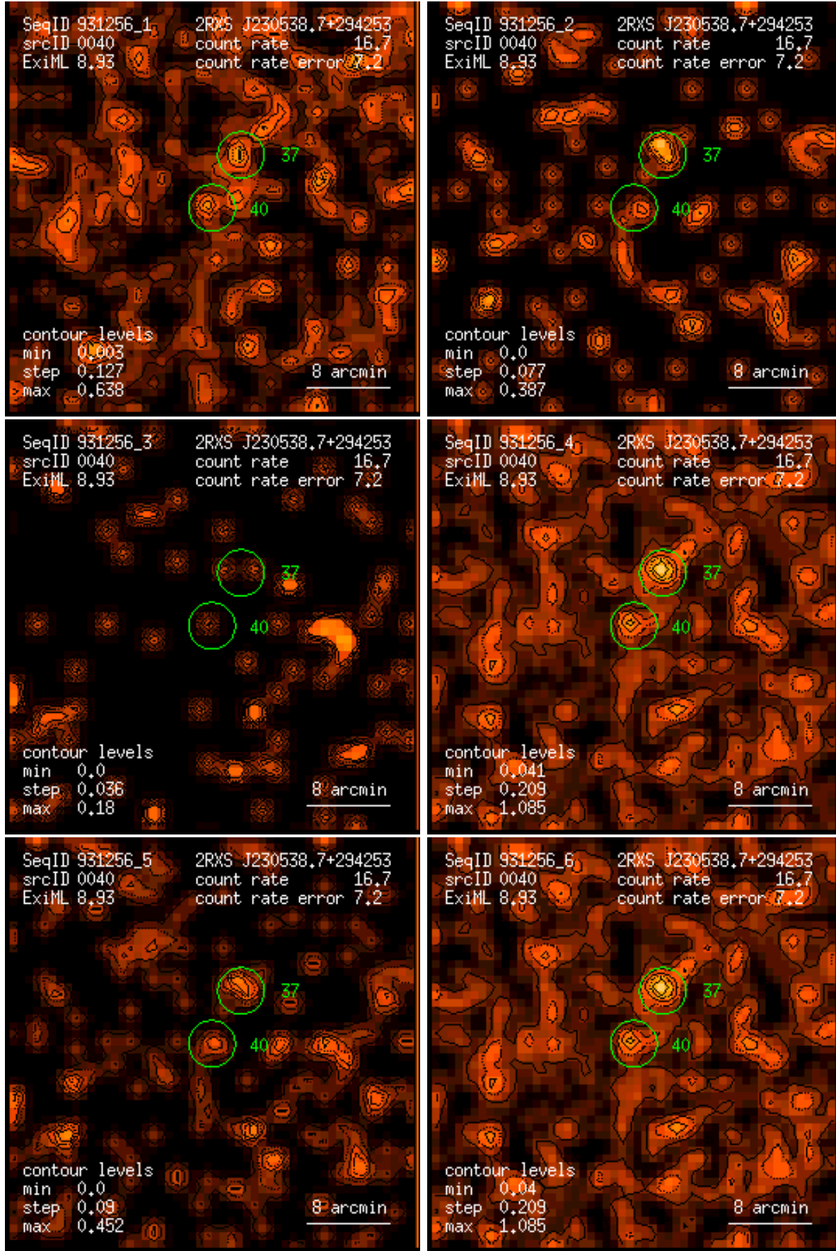
Figure 40: RASS 931256: detection 0040: band rate images, Gaussian filter: (1) PSPC channels 11 – 41, (2) 52 – 90, (3) 91 – 201, (4) 11 – 235, (5) 52 – 201, (6) 11 – 201. Broad band rates in counts/ks. Band rate contour levels in counts/ks/arcmin 2 .
